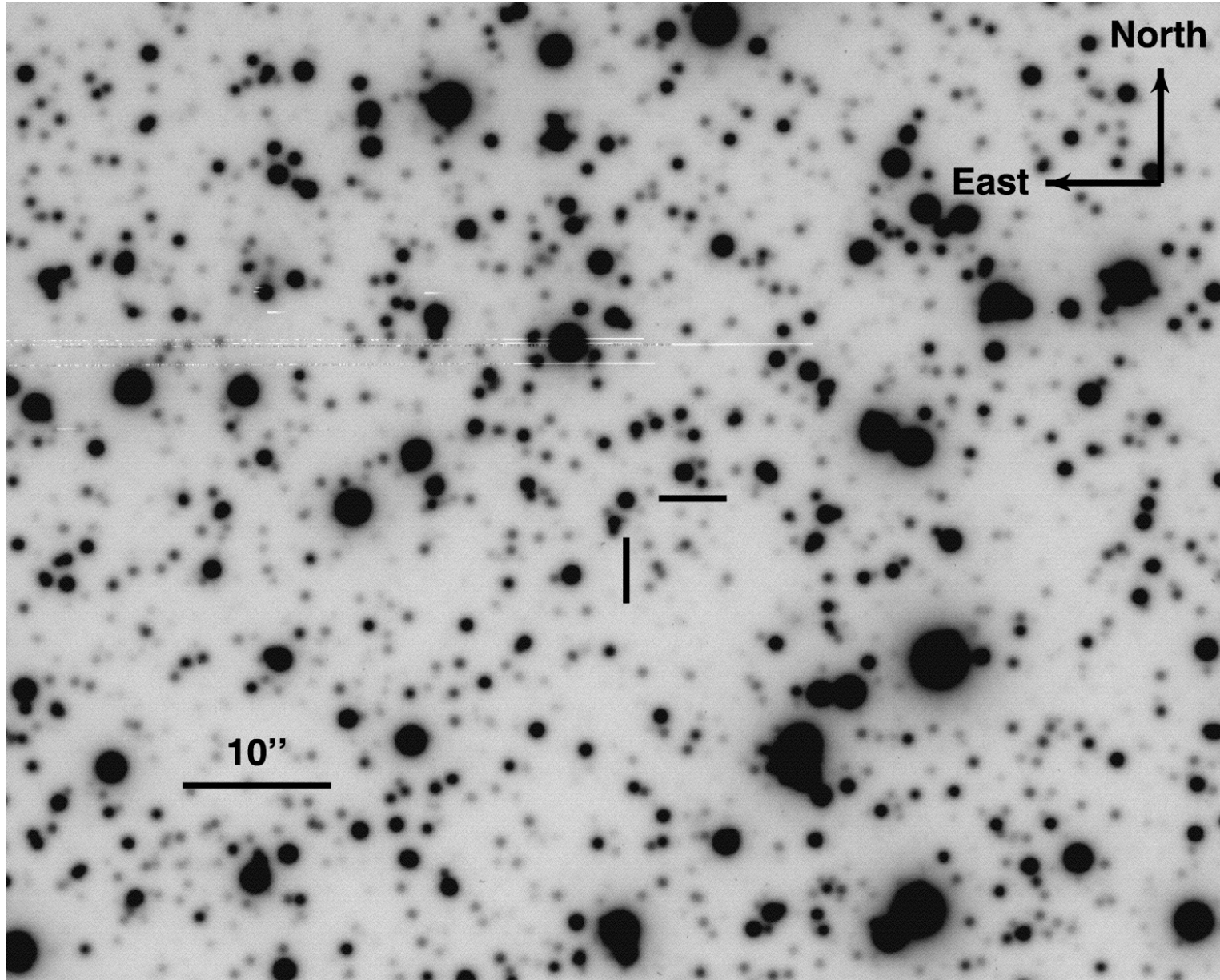
Fig. 1. from The XRay Position and Optical Counterpart of the Accretionpowered Millisecond Pulsar XTE J1814338 Krauss et al. 2005 ApJ 627 910 doi:10.1086/430595 https://dx.doi.org/10.1086/430595 © 2005. The American Astronomical Society. All rights reserved. Printed in U.S.A.
