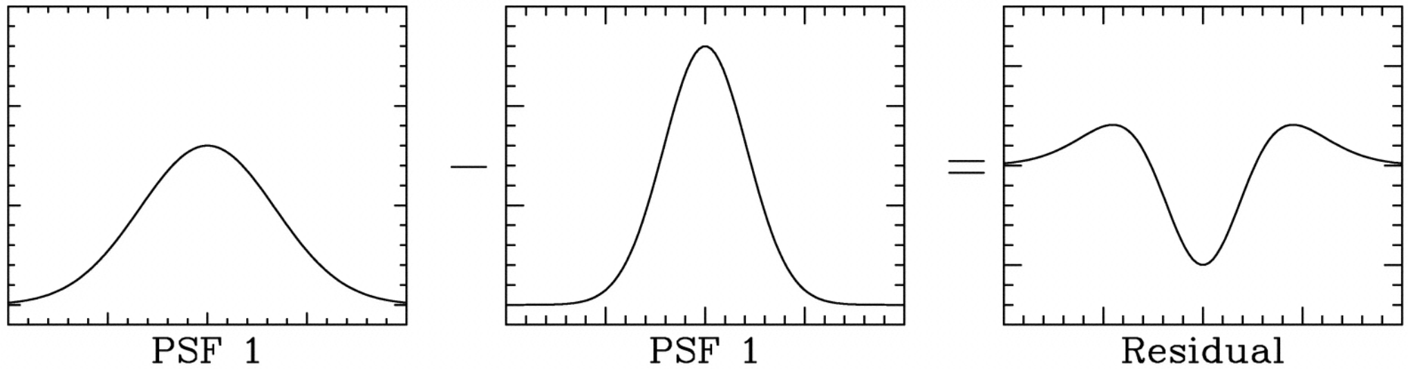
Fig. 9. from The Threedimensional Circumstellar Environment of SN 1987A Sugerman et al. 2005 ApJS 159 60 doi:10.1086/430408 https://dx.doi.org/10.1086/430408 © 2005. The American Astronomical Society. All rights reserved. Printed in U.S.A.
