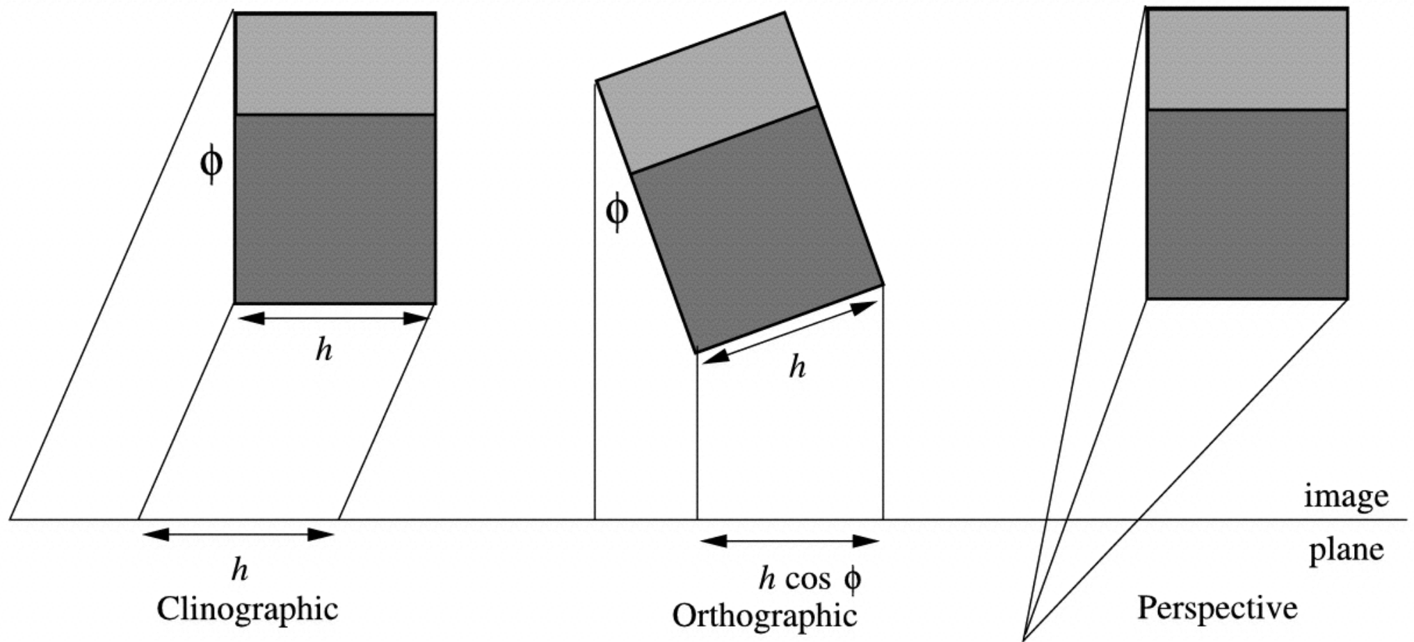
Fig. 49. from The Threedimensional Circumstellar Environment of SN 1987A Sugerman et al. 2005 ApJS 159 60 doi:10.1086/430408 https://dx.doi.org/10.1086/430408 © 2005. The American Astronomical Society. All rights reserved. Printed in U.S.A.
