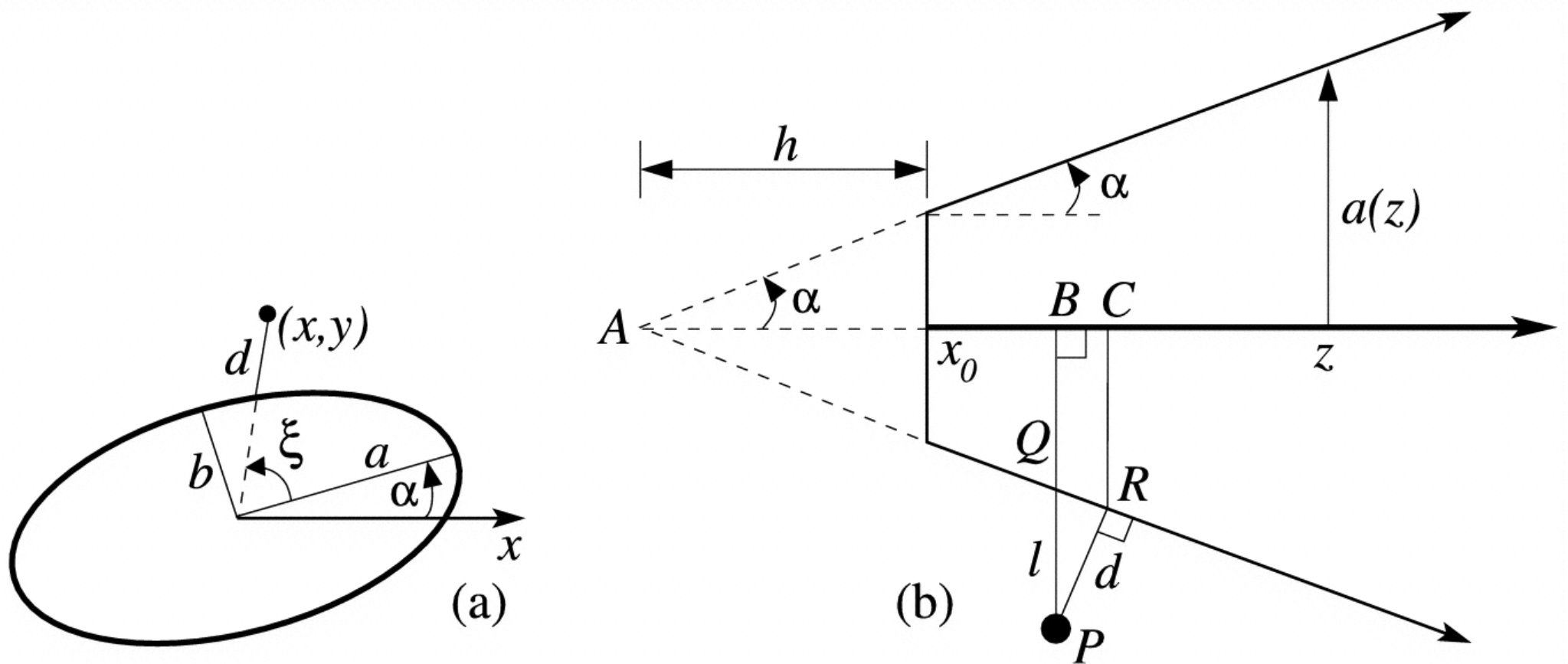
Fig. 48. from The Threedimensional Circumstellar Environment of SN 1987A Sugerman et al. 2005 ApJS 159 60 doi:10.1086/430408 https://dx.doi.org/10.1086/430408 © 2005. The American Astronomical Society. All rights reserved. Printed in U.S.A.
