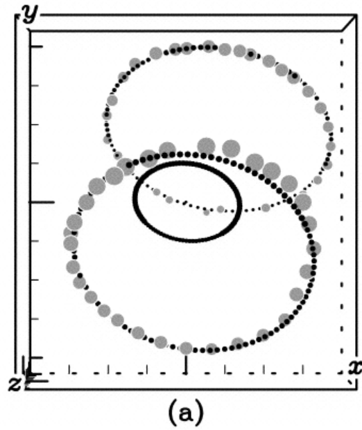
Fig. 42. from The Threedimensional Circumstellar Environment of SN 1987A Sugerman et al. 2005 ApJS 159 60 doi:10.1086/430408 https://dx.doi.org/10.1086/430408 © 2005. The American Astronomical Society. All rights reserved. Printed in U.S.A.
