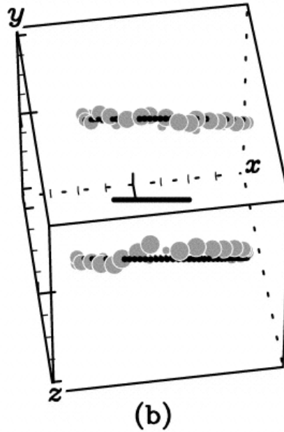
Fig. 42. from The Threedimensional Circumstellar Environment of SN 1987A Sugerman et al. 2005 ApJS 159 60 doi:10.1086/430408 https://dx.doi.org/10.1086/430408 © 2005. The American Astronomical Society. All rights reserved. Printed in U.S.A.
