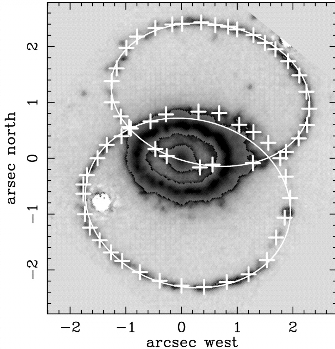
Fig. 40. from The Threedimensional Circumstellar Environment of SN 1987A Sugerman et al. 2005 ApJS 159 60 doi:10.1086/430408 https://dx.doi.org/10.1086/430408 © 2005. The American Astronomical Society. All rights reserved. Printed in U.S.A.
