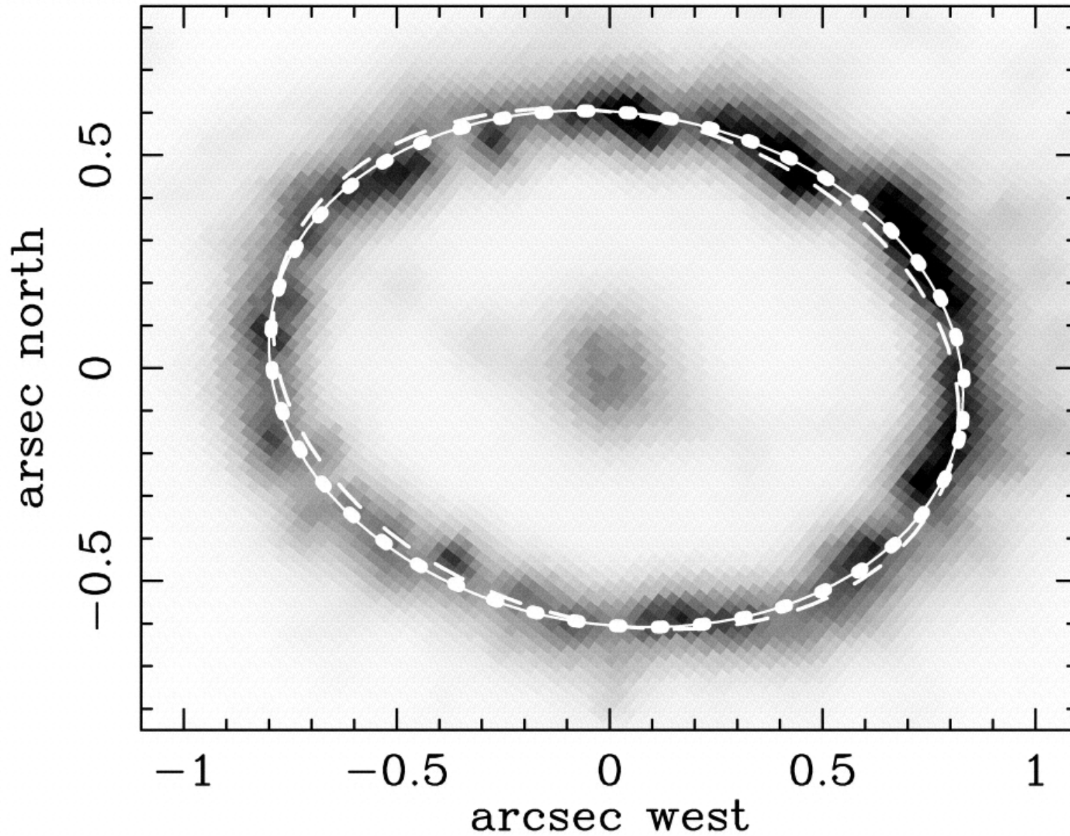
Fig. 37. from The Threedimensional Circumstellar Environment of SN 1987A Sugerman et al. 2005 ApJS 159 60 doi:10.1086/430408 https://dx.doi.org/10.1086/430408 © 2005. The American Astronomical Society. All rights reserved. Printed in U.S.A.
