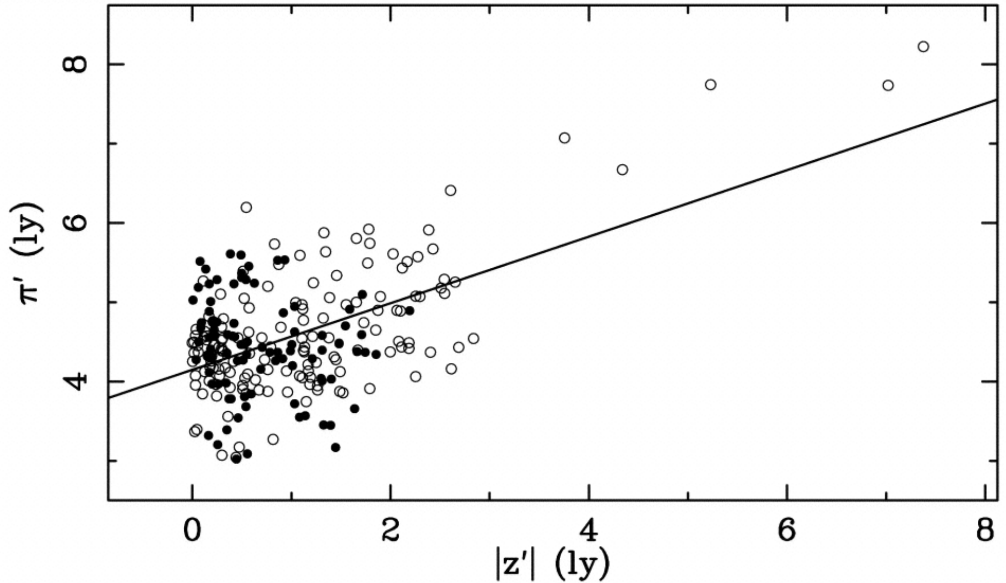
Fig. 30. from The Threedimensional Circumstellar Environment of SN 1987A Sugerman et al. 2005 ApJS 159 60 doi:10.1086/430408 https://dx.doi.org/10.1086/430408 © 2005. The American Astronomical Society. All rights reserved. Printed in U.S.A.
