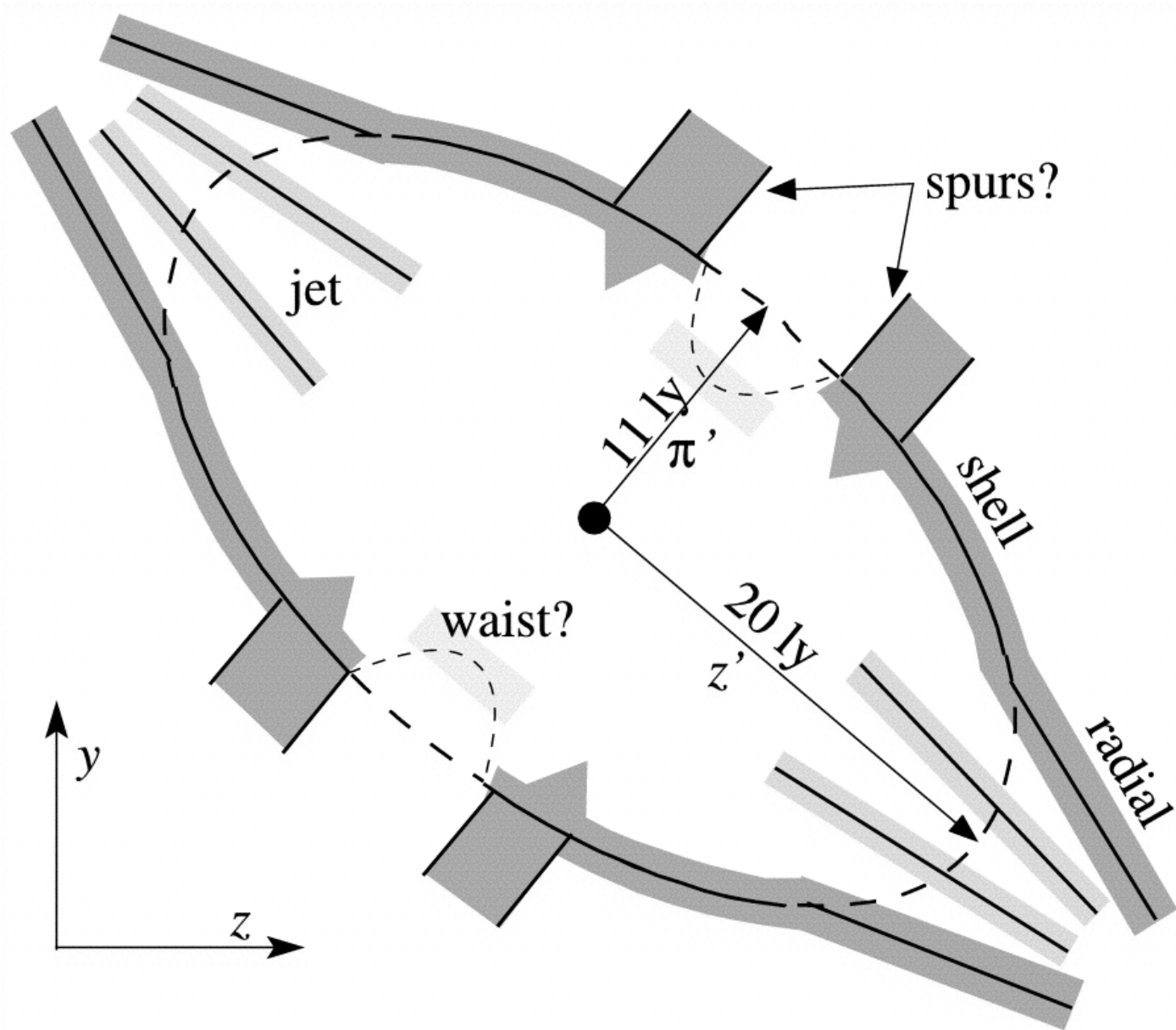
Fig. 27. from The Threedimensional Circumstellar Environment of SN 1987A Sugerman et al. 2005 ApJS 159 60 doi:10.1086/430408 https://dx.doi.org/10.1086/430408 © 2005. The American Astronomical Society. All rights reserved. Printed in U.S.A.
