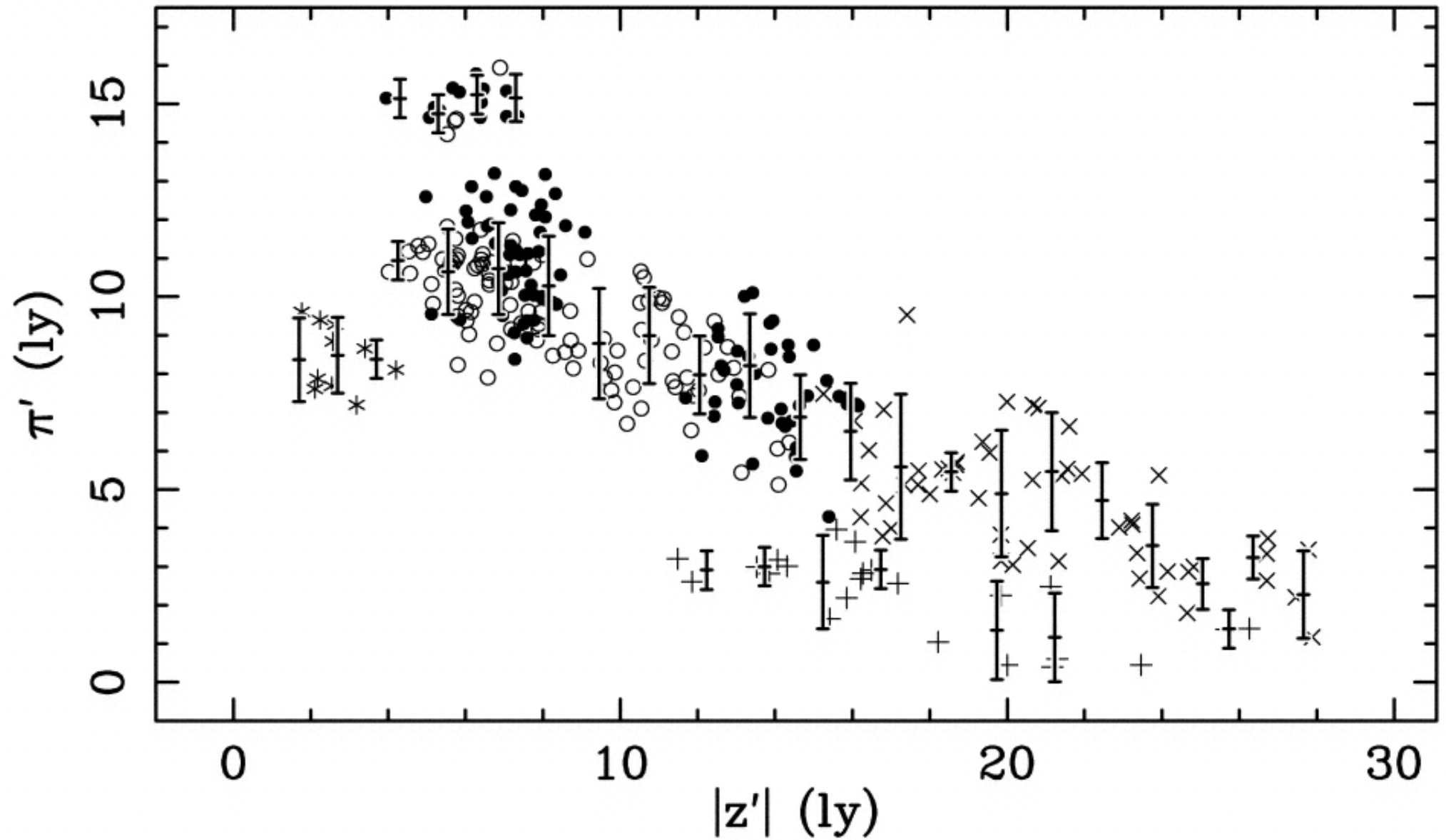
Fig. 26. from The Threedimensional Circumstellar Environment of SN 1987A Sugerman et al. 2005 ApJS 159 60 doi:10.1086/430408 https://dx.doi.org/10.1086/430408 © 2005. The American Astronomical Society. All rights reserved. Printed in U.S.A.
