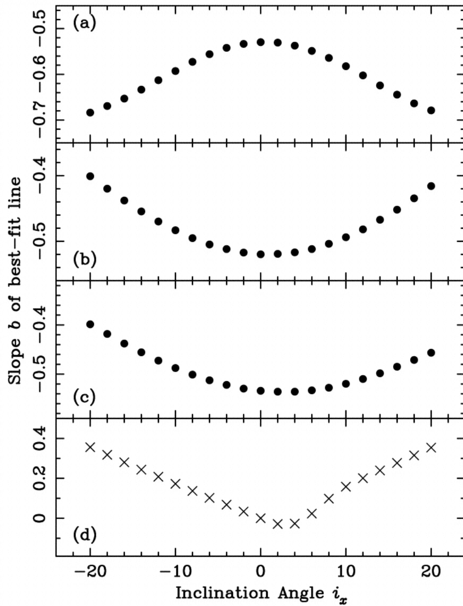
Fig. 23. from The Threedimensional Circumstellar Environment of SN 1987A Sugerman et al. 2005 ApJS 159 60 doi:10.1086/430408 https://dx.doi.org/10.1086/430408 © 2005. The American Astronomical Society. All rights reserved. Printed in U.S.A.
