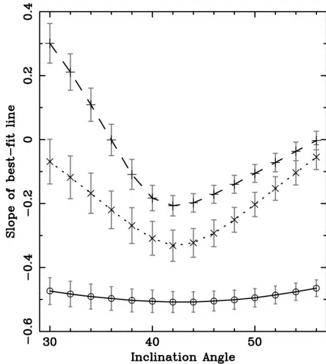
Fig. 21. from The Threedimensional Circumstellar Environment of SN 1987A Sugerman et al. 2005 ApJS 159 60 doi:10.1086/430408 https://dx.doi.org/10.1086/430408 © 2005. The American Astronomical Society. All rights reserved. Printed in U.S.A.
