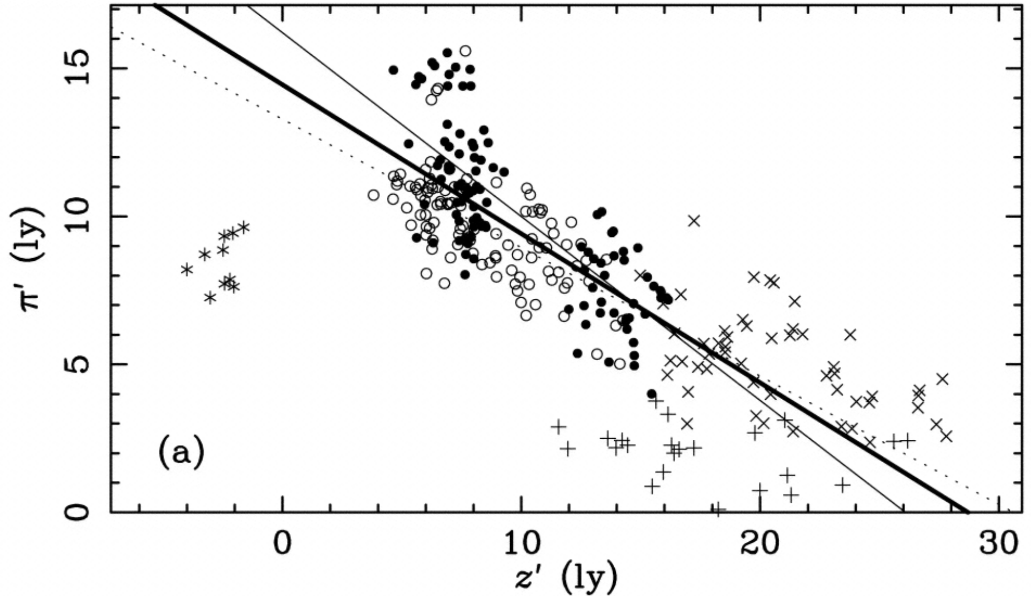
Fig. 19. from The Threedimensional Circumstellar Environment of SN 1987A Sugerman et al. 2005 ApJS 159 60 doi:10.1086/430408 https://dx.doi.org/10.1086/430408 © 2005. The American Astronomical Society. All rights reserved. Printed in U.S.A.
