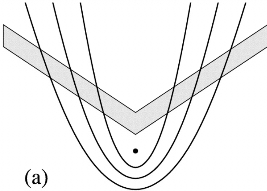
Fig. 17. from The Threedimensional Circumstellar Environment of SN 1987A Sugerman et al. 2005 ApJS 159 60 doi:10.1086/430408 https://dx.doi.org/10.1086/430408 © 2005. The American Astronomical Society. All rights reserved. Printed in U.S.A.
