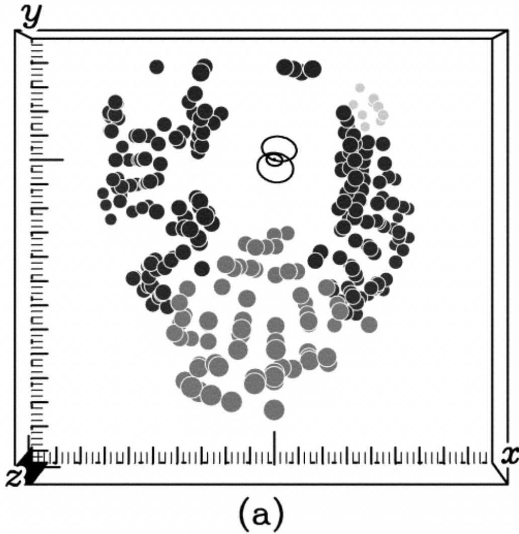
Fig. 16. from The Threedimensional Circumstellar Environment of SN 1987A Sugerman et al. 2005 ApJS 159 60 doi:10.1086/430408 https://dx.doi.org/10.1086/430408 © 2005. The American Astronomical Society. All rights reserved. Printed in U.S.A.
