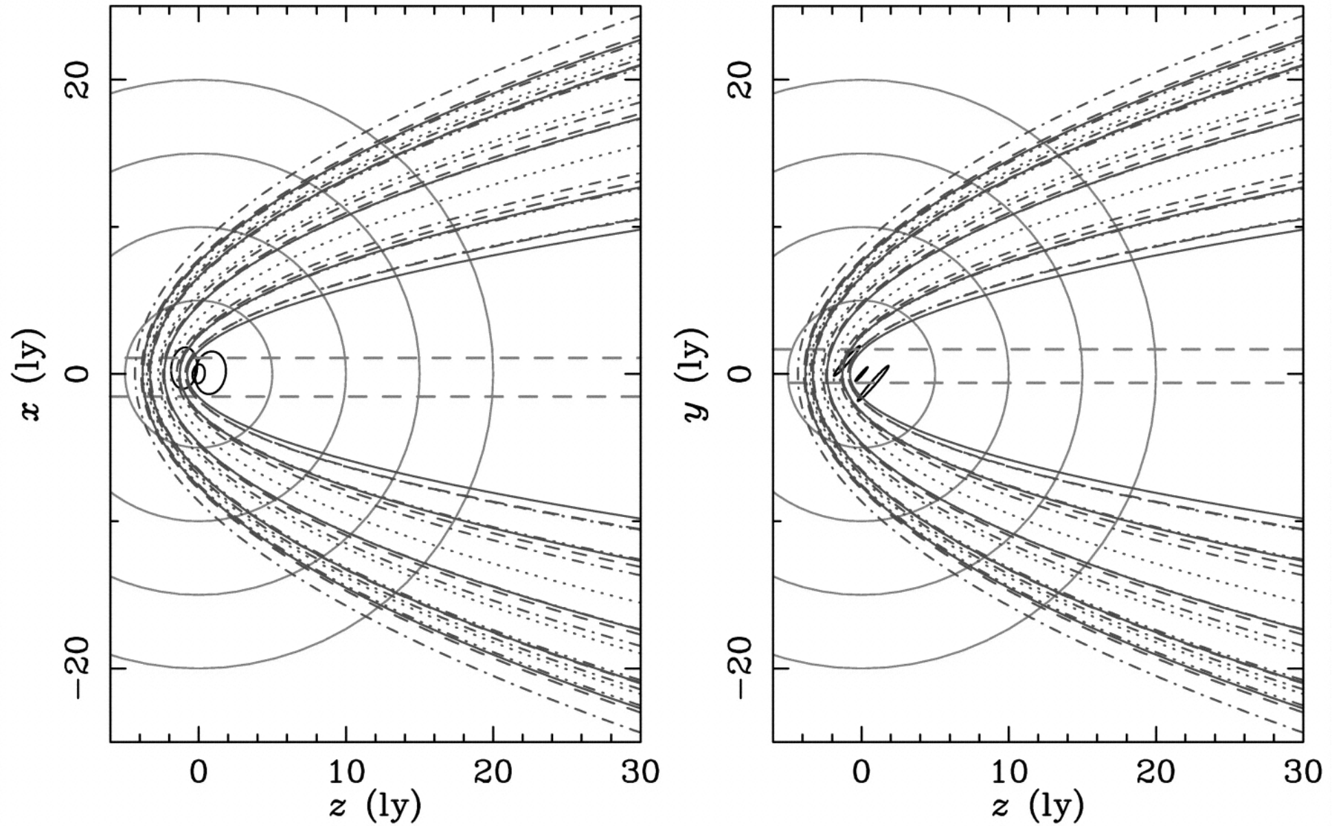
Fig. 14. from The Threedimensional Circumstellar Environment of SN 1987A Sugerman et al. 2005 ApJS 159 60 doi:10.1086/430408 https://dx.doi.org/10.1086/430408 © 2005. The American Astronomical Society. All rights reserved. Printed in U.S.A.
