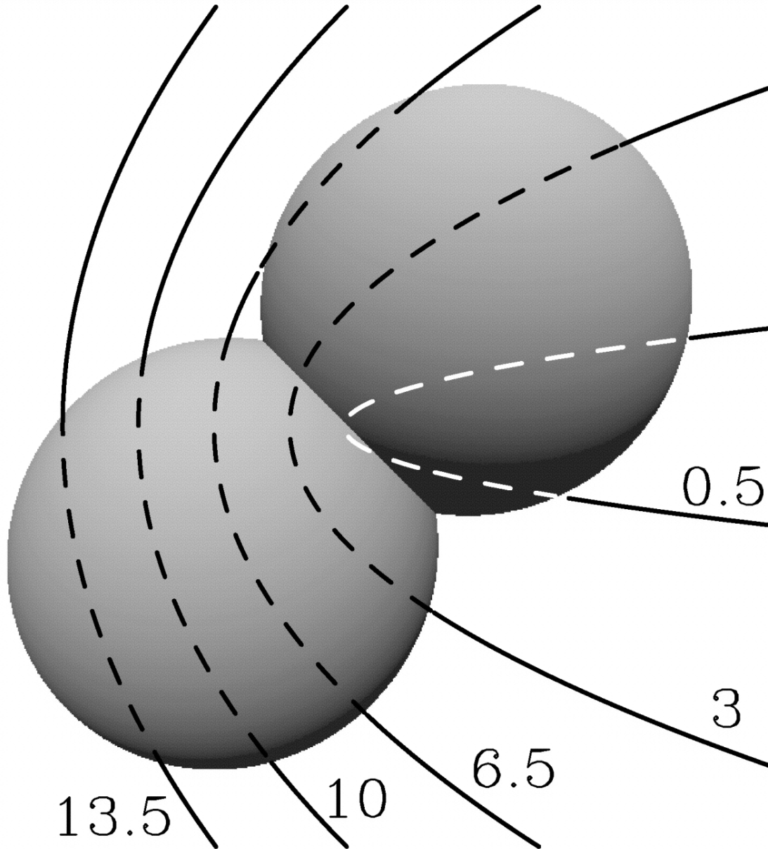
Fig. 13. from The Threedimensional Circumstellar Environment of SN 1987A Sugerman et al. 2005 ApJS 159 60 doi:10.1086/430408 https://dx.doi.org/10.1086/430408 © 2005. The American Astronomical Society. All rights reserved. Printed in U.S.A.
