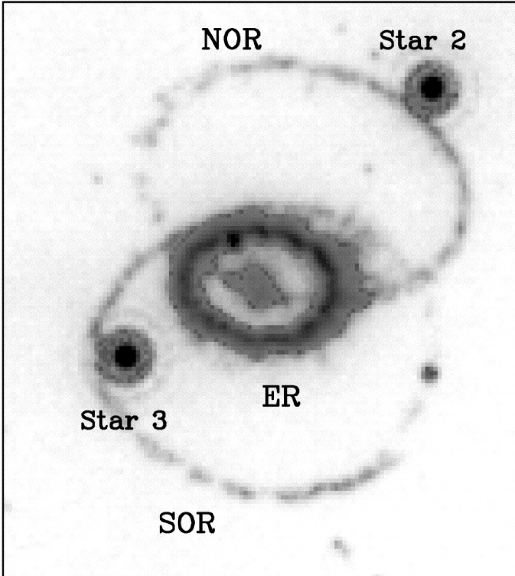
Fig. 1. from The Threedimensional Circumstellar Environment of SN 1987A Sugerman et al. 2005 ApJS 159 60 doi:10.1086/430408 https://dx.doi.org/10.1086/430408 © 2005. The American Astronomical Society. All rights reserved. Printed in U.S.A.
