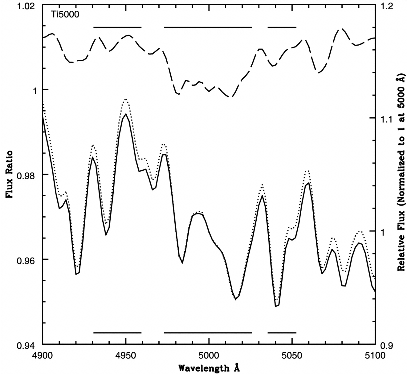
Fig. 9. from The Observability of Abundance Ratio Effects in Dynamically Hot Stellar Systems Serven, Worthey, & Briley 2005 ApJ 627 754 doi:10.1086/430400 https://dx.doi.org/10.1086/430400 © 2005. The American Astronomical Society. All rights reserved. Printed in U.S.A.
