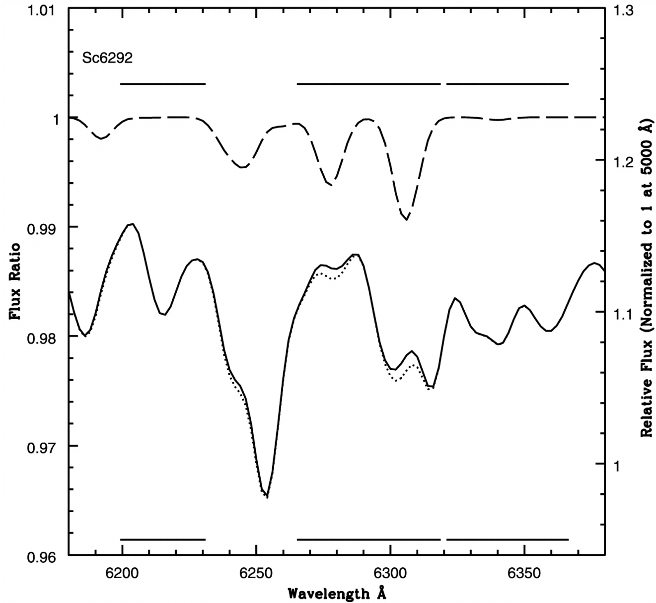
Fig. 8. from The Observability of Abundance Ratio Effects in Dynamically Hot Stellar Systems Serven, Worthey, & Briley 2005 ApJ 627 754 doi:10.1086/430400 https://dx.doi.org/10.1086/430400 © 2005. The American Astronomical Society. All rights reserved. Printed in U.S.A.
