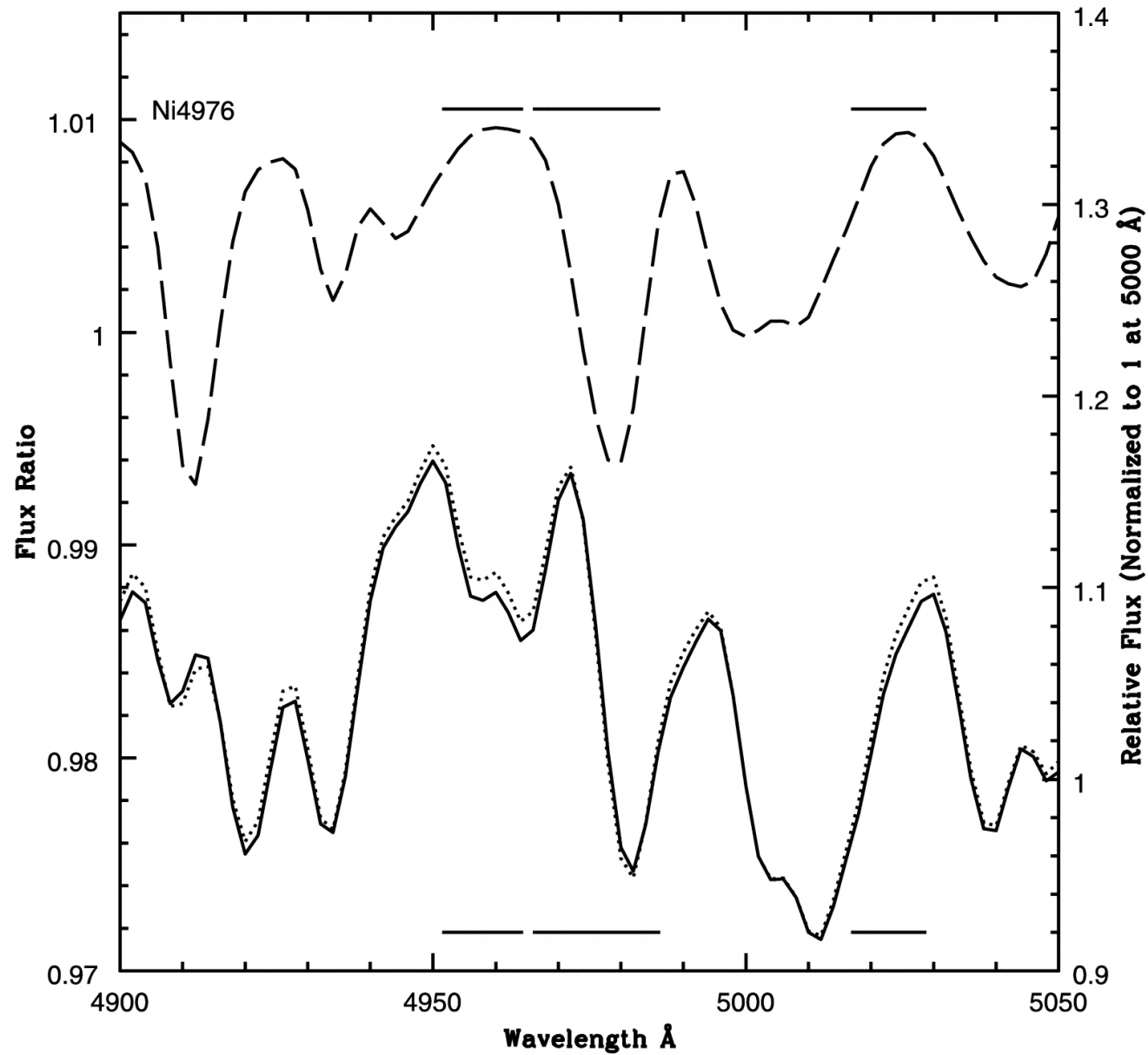
Fig. 7. from The Observability of Abundance Ratio Effects in Dynamically Hot Stellar Systems Serven, Worthey, & Briley 2005 ApJ 627 754 doi:10.1086/430400 https://dx.doi.org/10.1086/430400 © 2005. The American Astronomical Society. All rights reserved. Printed in U.S.A.
