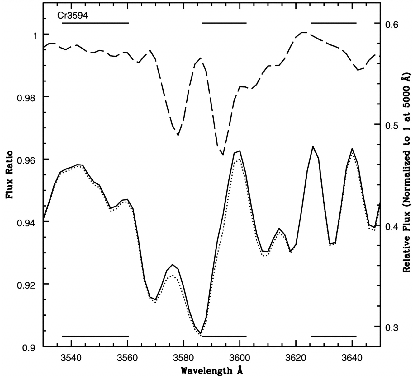
Fig. 6. from The Observability of Abundance Ratio Effects in Dynamically Hot Stellar Systems Serven, Worthey, & Briley 2005 ApJ 627 754 doi:10.1086/430400 https://dx.doi.org/10.1086/430400 © 2005. The American Astronomical Society. All rights reserved. Printed in U.S.A.
