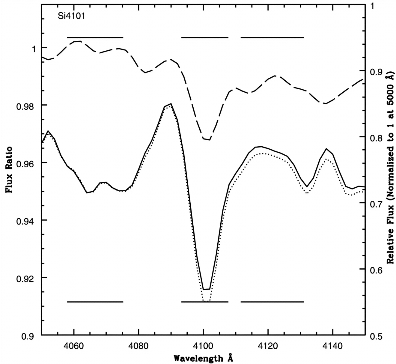
Fig. 5. from The Observability of Abundance Ratio Effects in Dynamically Hot Stellar Systems Serven, Worthey, & Briley 2005 ApJ 627 754 doi:10.1086/430400 https://dx.doi.org/10.1086/430400 © 2005. The American Astronomical Society. All rights reserved. Printed in U.S.A.
