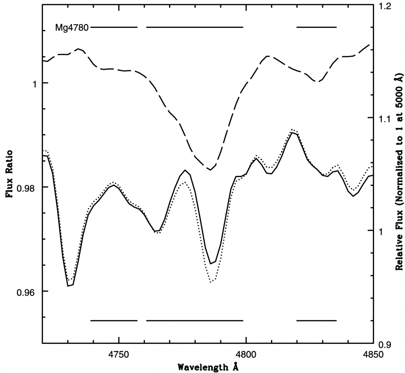
Fig. 4. from The Observability of Abundance Ratio Effects in Dynamically Hot Stellar Systems Serven, Worthey, & Briley 2005 ApJ 627 754 doi:10.1086/430400 https://dx.doi.org/10.1086/430400 © 2005. The American Astronomical Society. All rights reserved. Printed in U.S.A.
