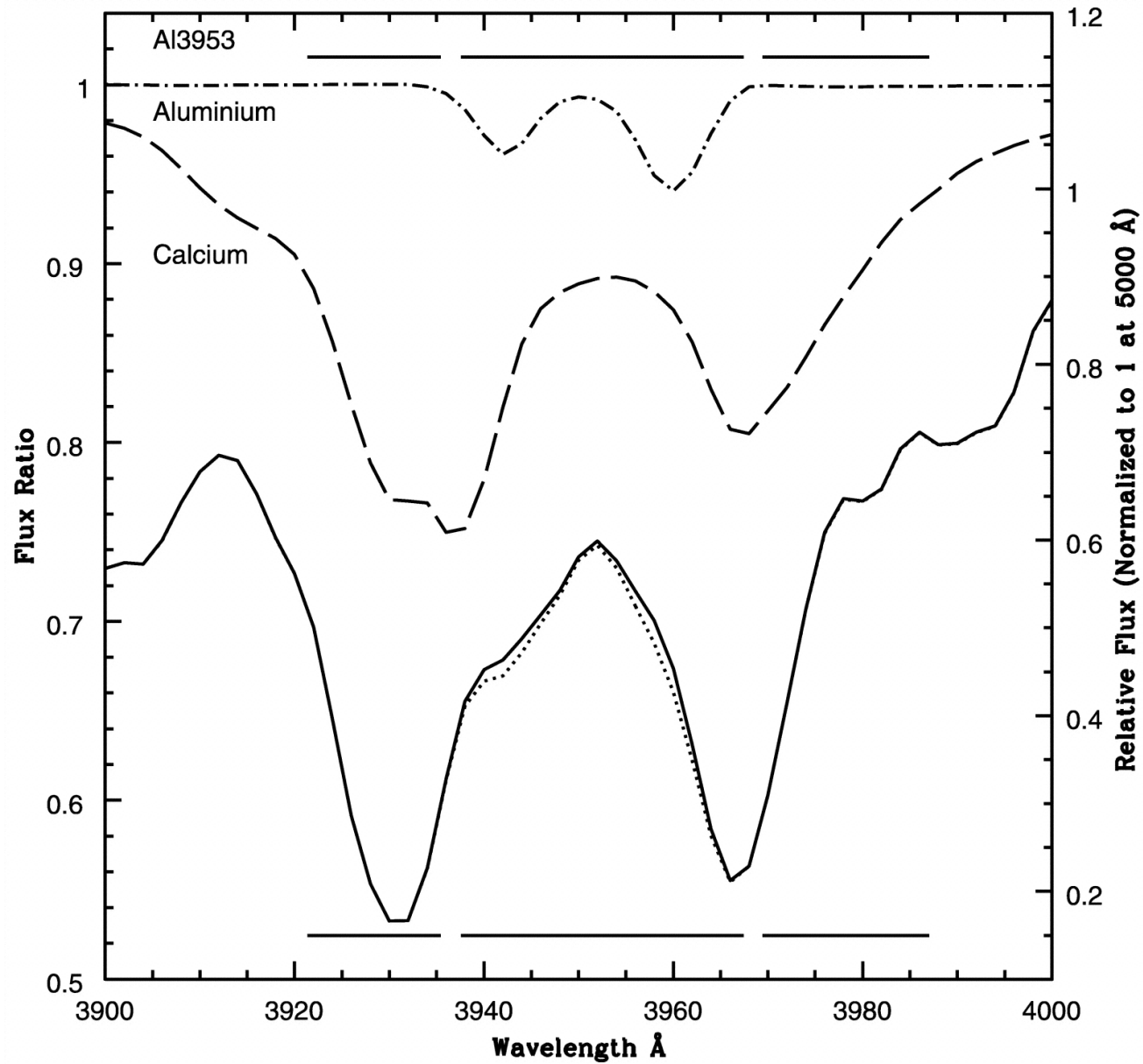
Fig. 3. from The Observability of Abundance Ratio Effects in Dynamically Hot Stellar Systems Serven, Worthey, & Briley 2005 ApJ 627 754 doi:10.1086/430400 https://dx.doi.org/10.1086/430400 © 2005. The American Astronomical Society. All rights reserved. Printed in U.S.A.
