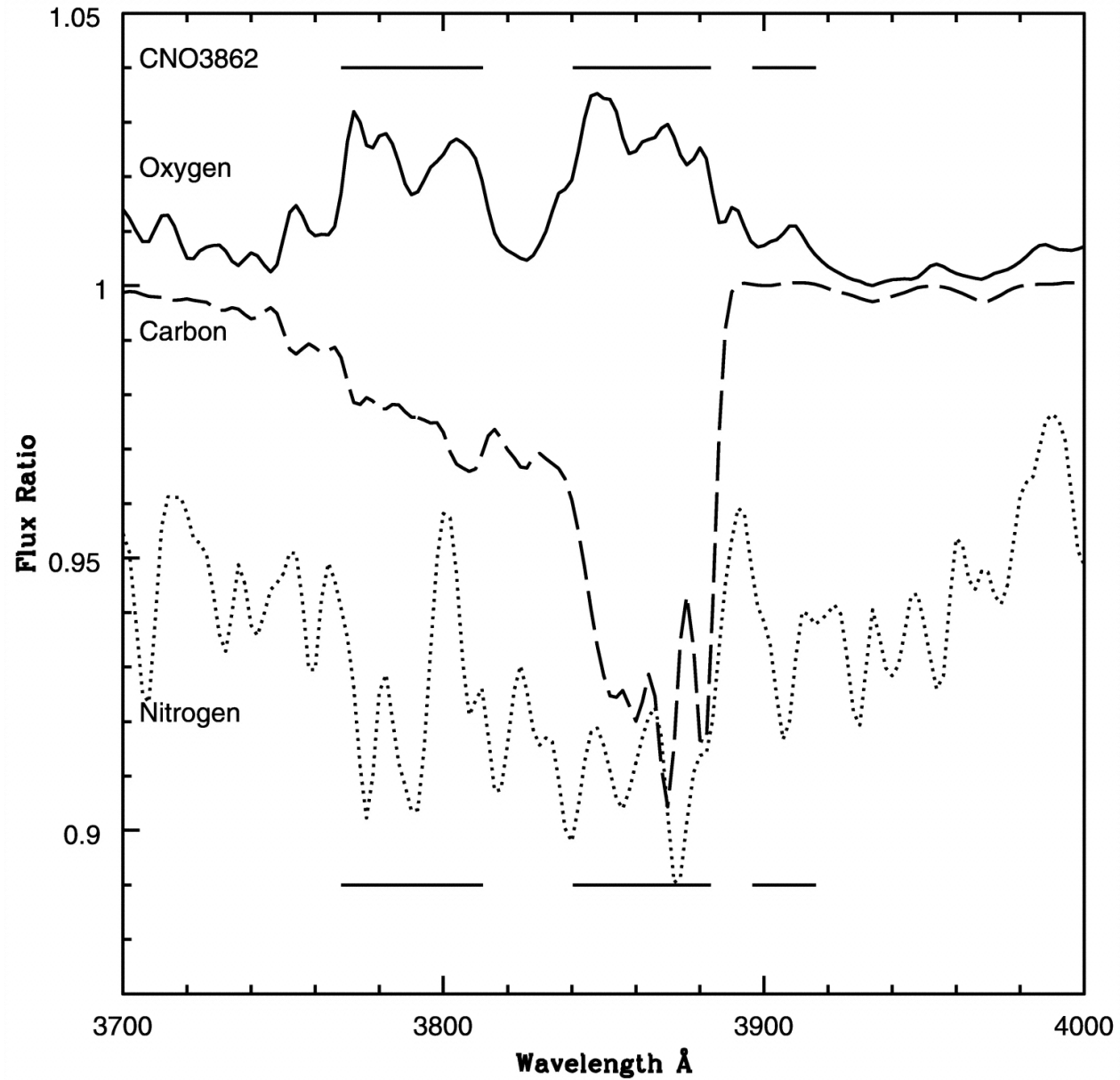
Fig. 2. from The Observability of Abundance Ratio Effects in Dynamically Hot Stellar Systems Serven, Worthey, & Briley 2005 ApJ 627 754 doi:10.1086/430400 https://dx.doi.org/10.1086/430400 © 2005. The American Astronomical Society. All rights reserved. Printed in U.S.A.
