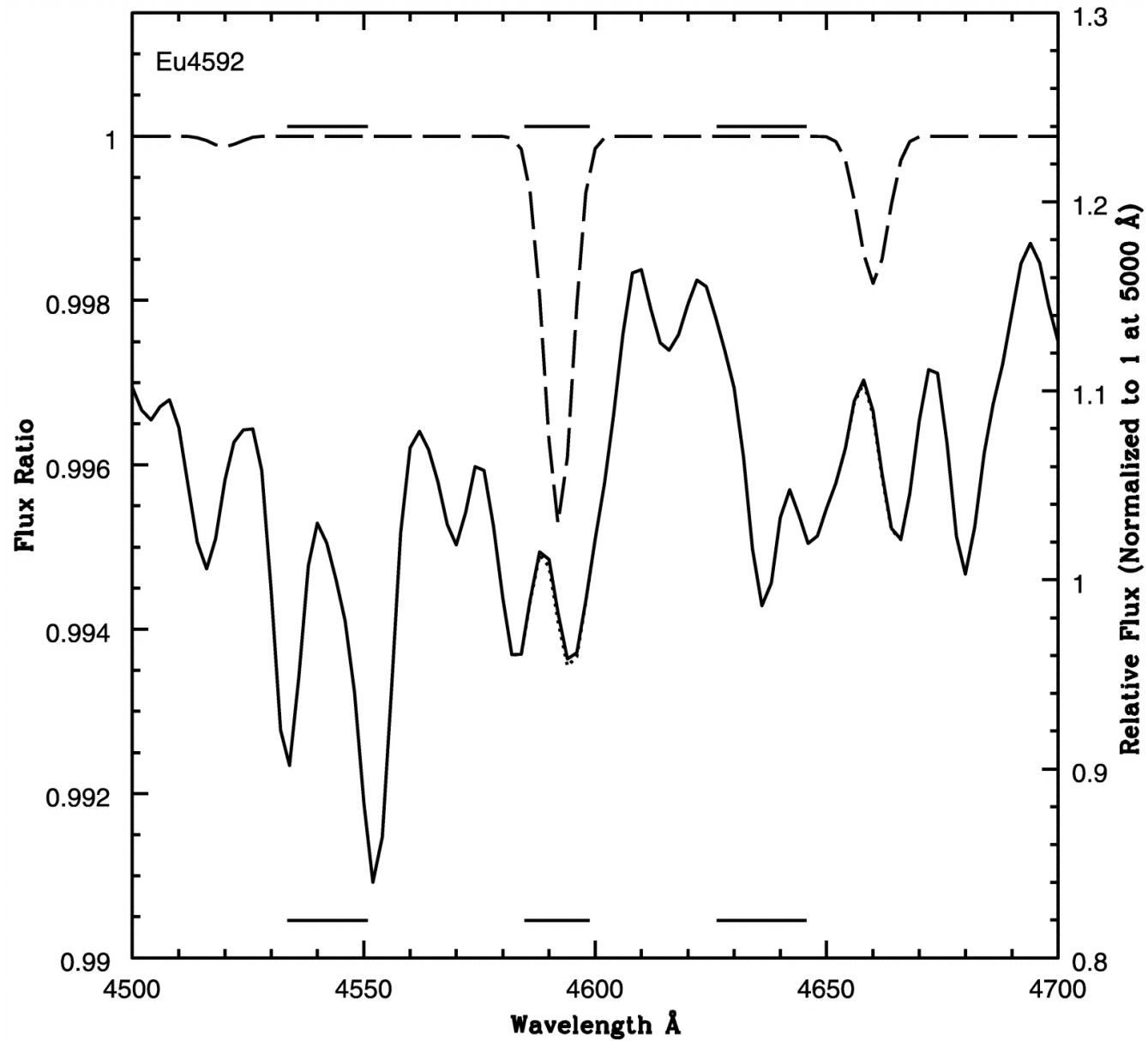
Fig. 14. from The Observability of Abundance Ratio Effects in Dynamically Hot Stellar Systems Serven, Worthey, & Briley 2005 ApJ 627 754 doi:10.1086/430400 https://dx.doi.org/10.1086/430400 © 2005. The American Astronomical Society. All rights reserved. Printed in U.S.A.
