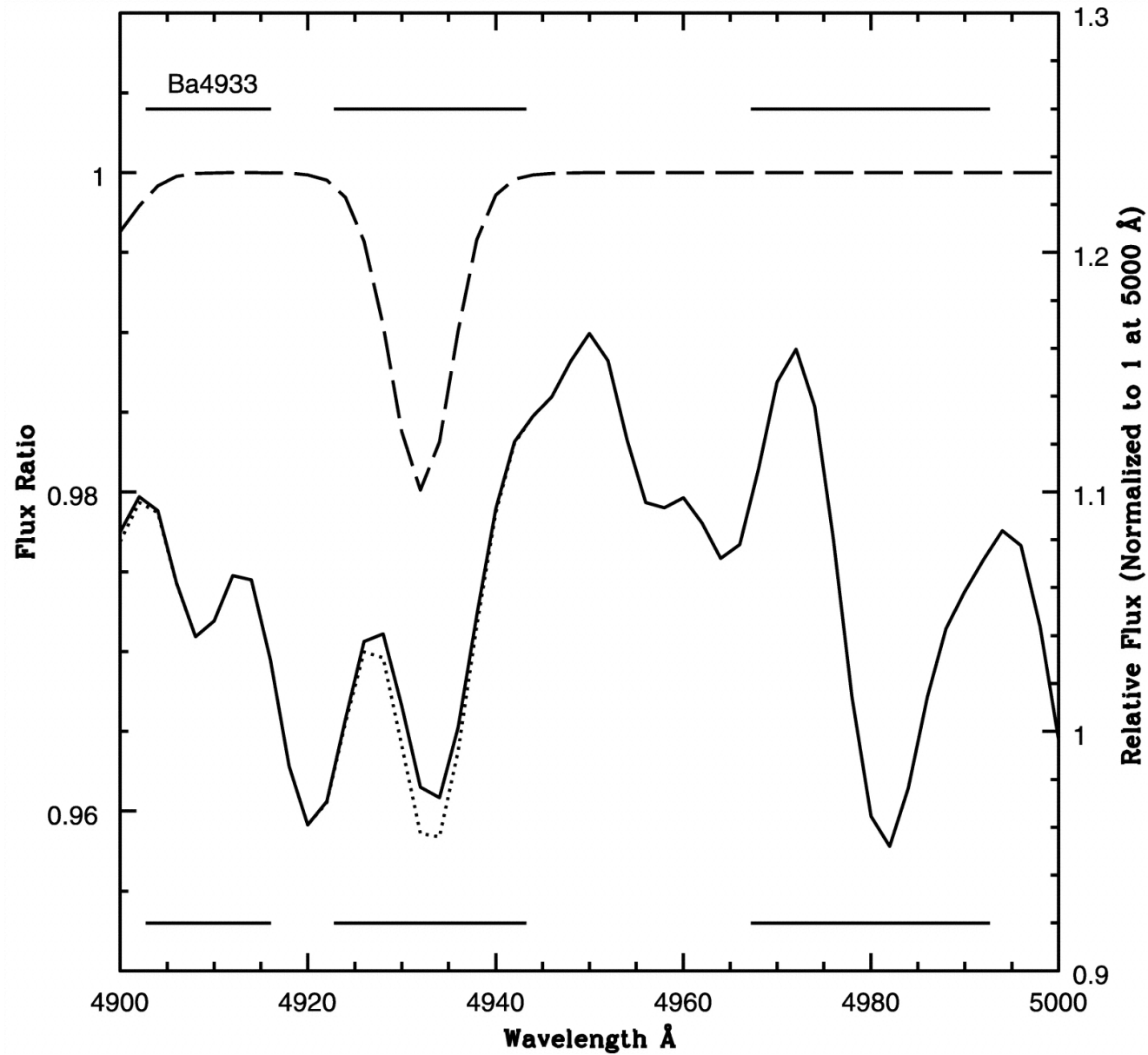
Fig. 13. from The Observability of Abundance Ratio Effects in Dynamically Hot Stellar Systems Serven, Worthey, & Briley 2005 ApJ 627 754 doi:10.1086/430400 https://dx.doi.org/10.1086/430400 © 2005. The American Astronomical Society. All rights reserved. Printed in U.S.A.
