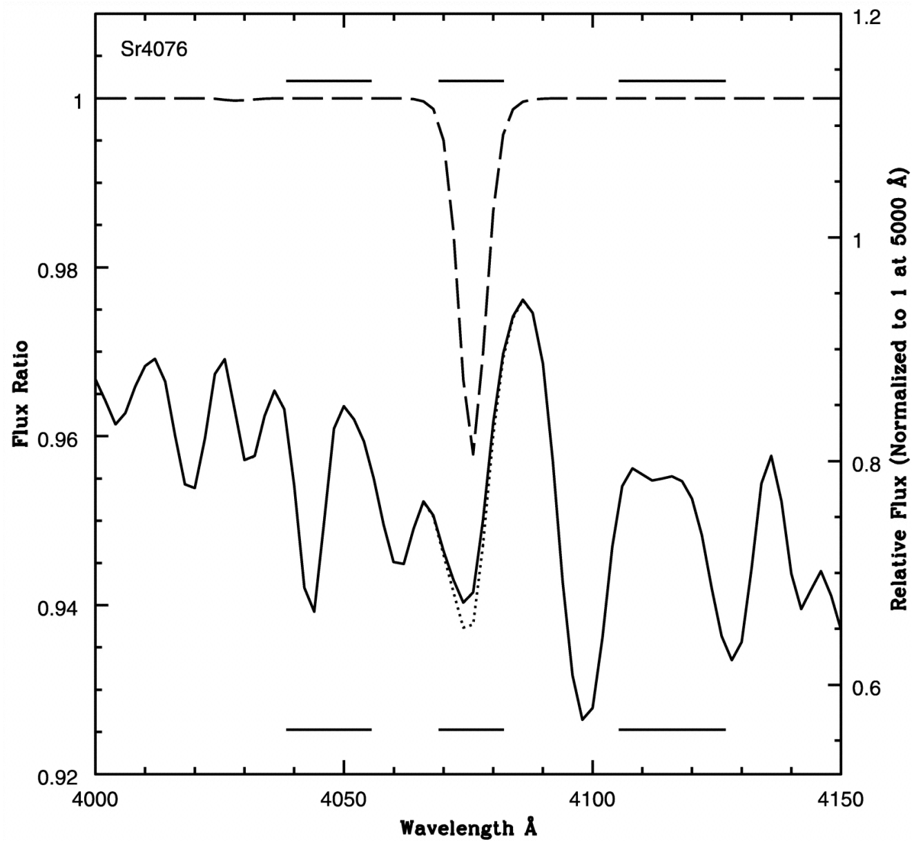
Fig. 12. from The Observability of Abundance Ratio Effects in Dynamically Hot Stellar Systems Serven, Worthey, & Briley 2005 ApJ 627 754 doi:10.1086/430400 https://dx.doi.org/10.1086/430400 © 2005. The American Astronomical Society. All rights reserved. Printed in U.S.A.
