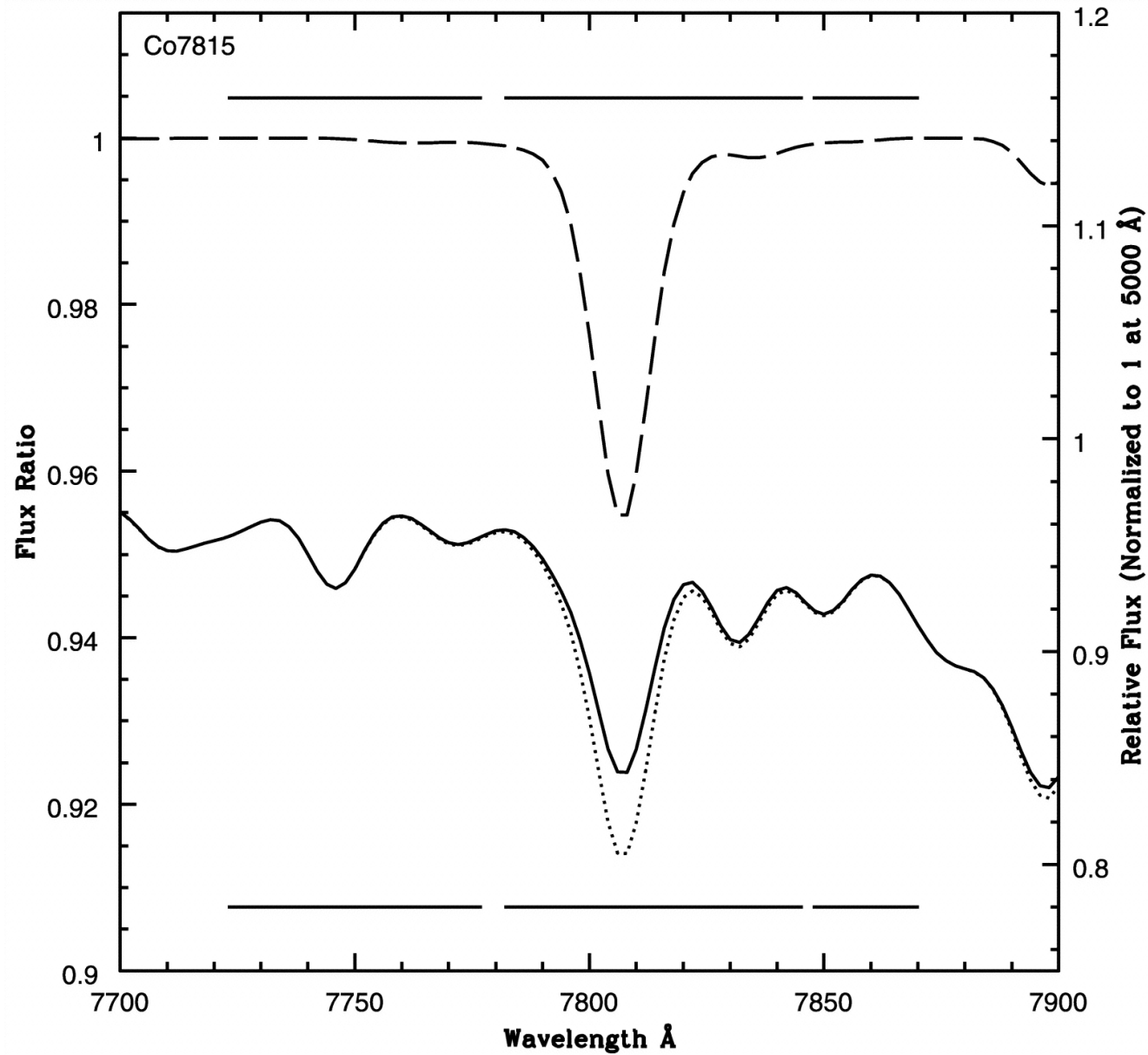
Fig. 11. from The Observability of Abundance Ratio Effects in Dynamically Hot Stellar Systems Serven, Worthey, & Briley 2005 ApJ 627 754 doi:10.1086/430400 https://dx.doi.org/10.1086/430400 © 2005. The American Astronomical Society. All rights reserved. Printed in U.S.A.
