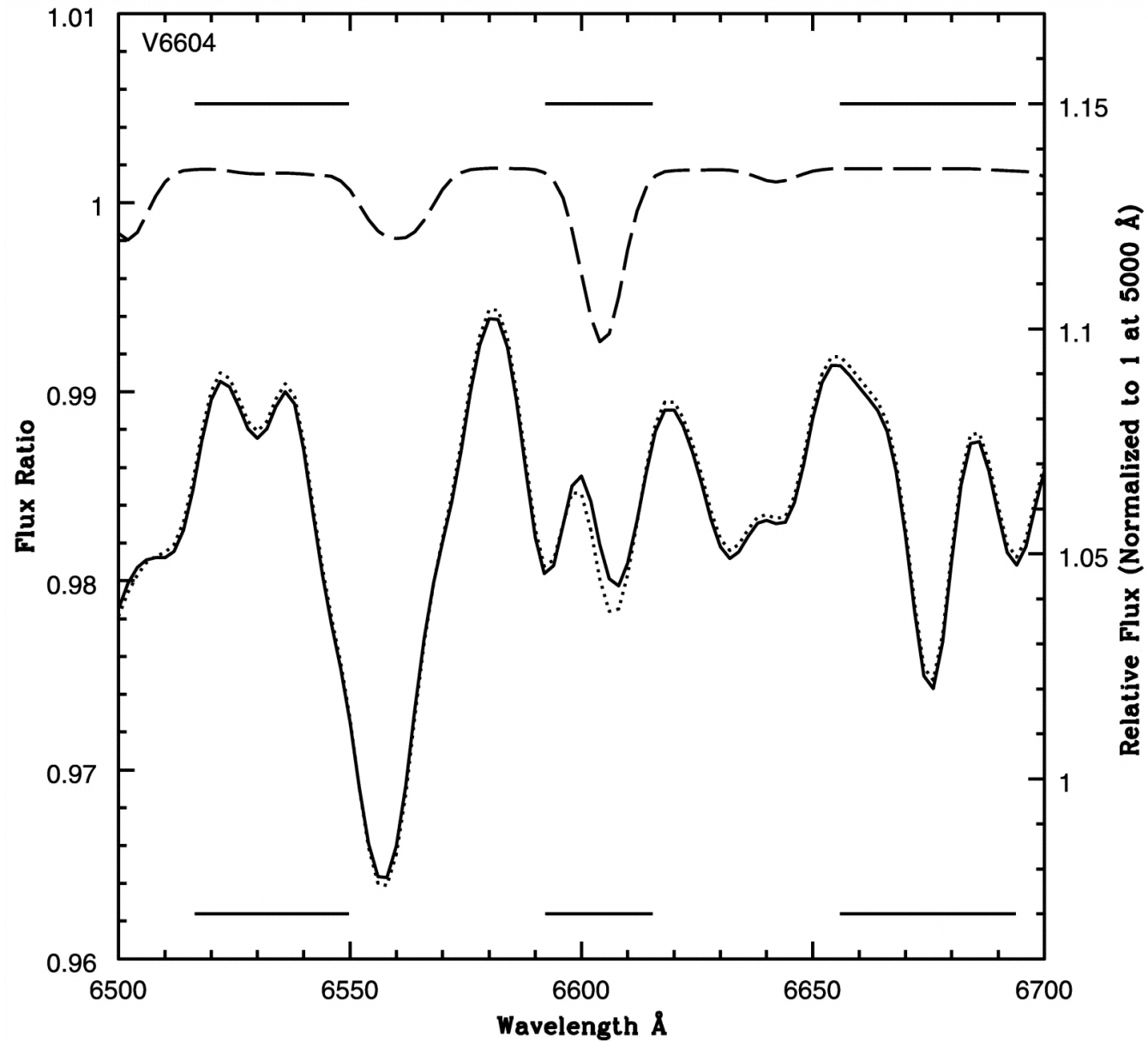
Fig. 10. from The Observability of Abundance Ratio Effects in Dynamically Hot Stellar Systems Seren, Worthey, & Briley 2005 ApJ 627 754 doi:10.1086/430400 https://dx.doi.org/10.1086/430400 © 2005. The American Astronomical Society. All rights reserved. Printed in U.S.A.
