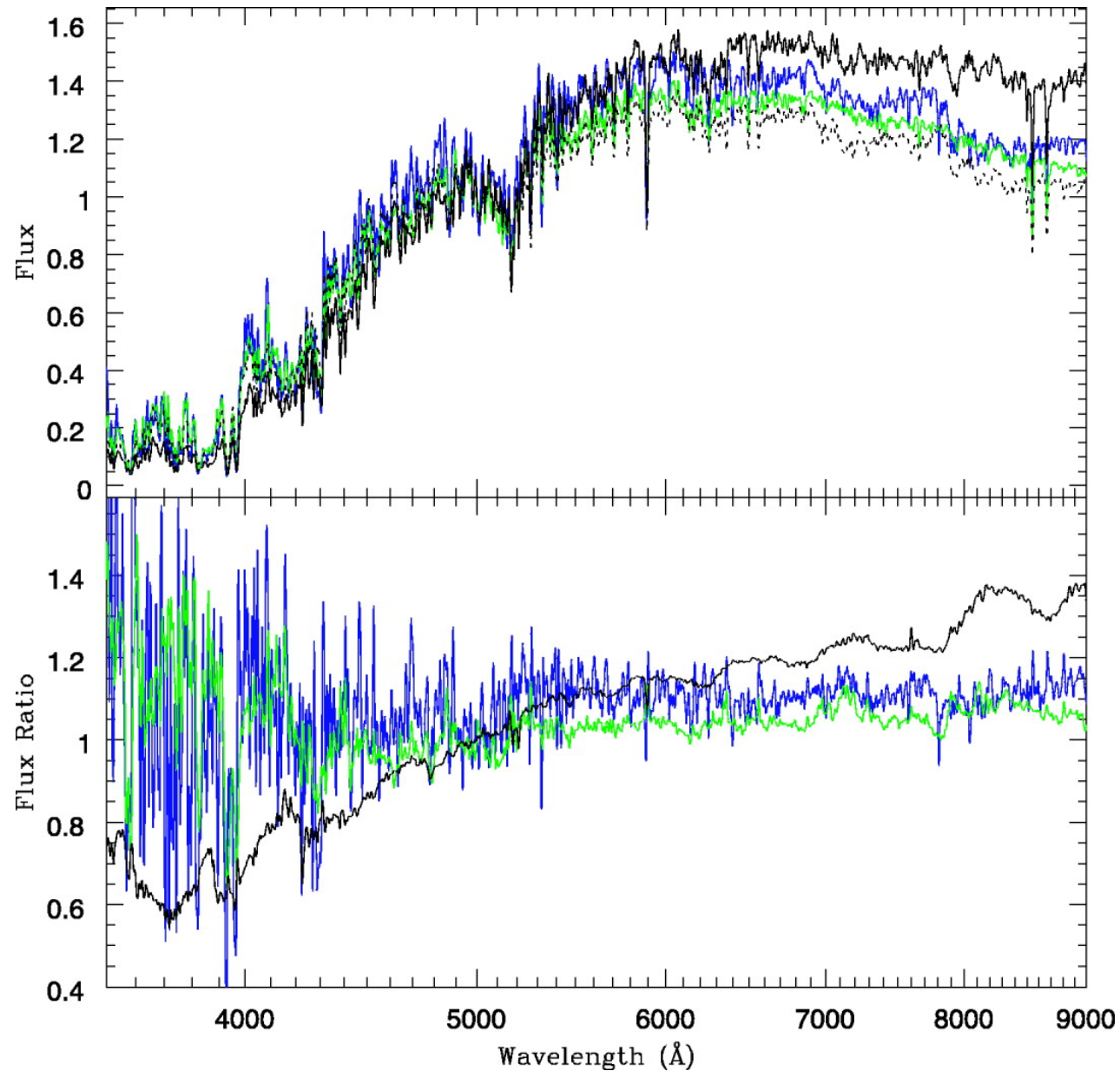
Fig. 1. from The Observability of Abundance Ratio Effects in Dynamically Hot Stellar Systems Serven, Worthey, & Briley 2005 ApJ 627 754 doi:10.1086/430400 https://dx.doi.org/10.1086/430400
