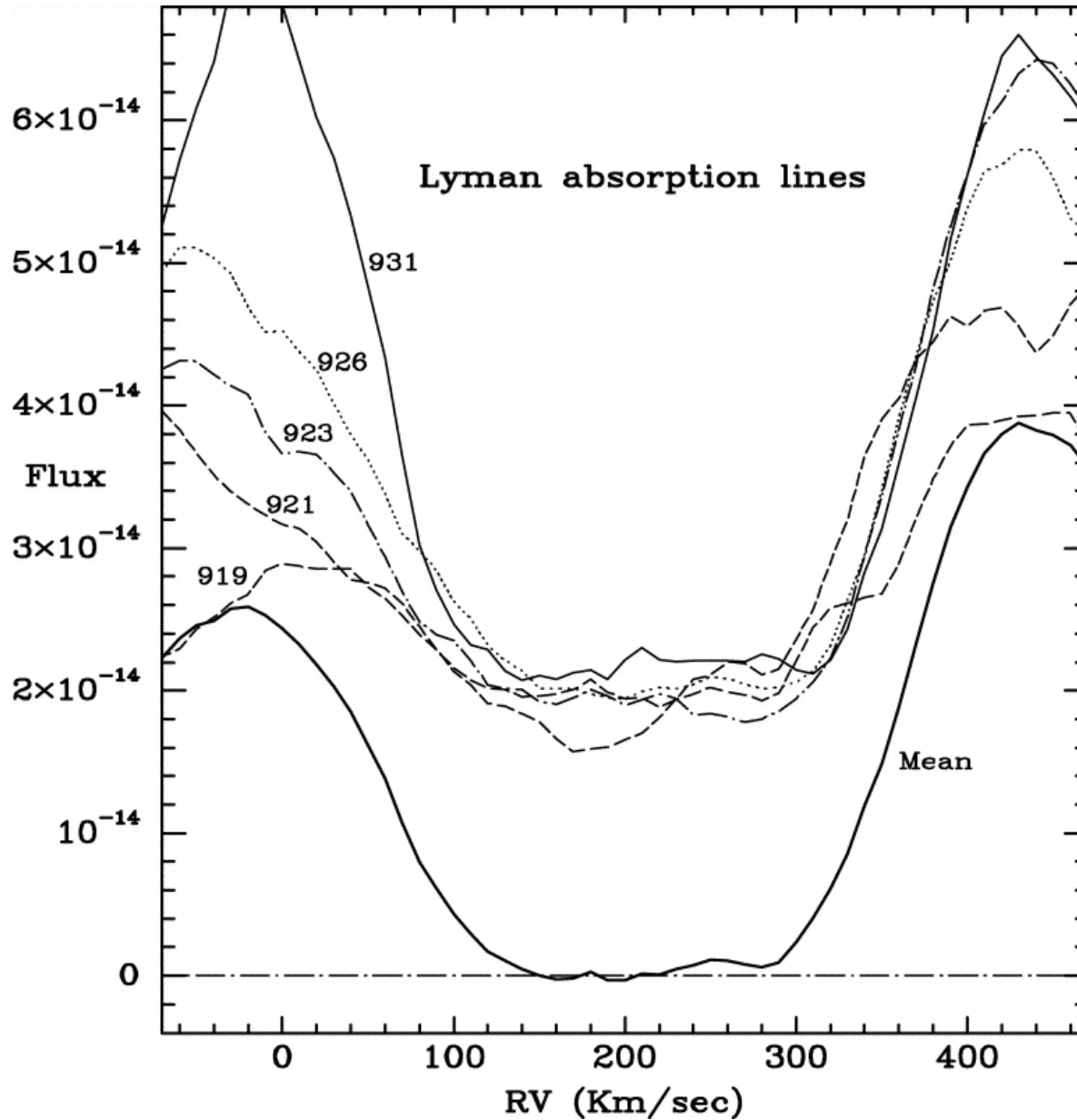
Fig. 6. from Far Ultraviolet Spectroscopic Explorer Observations of RX J0513.96951 Hutchings et al. 2005 AJ 129 2792 doi:10.1086/430147 https://dx.doi.org/10.1086/430147 © 2005. The American Astronomical Society. All rights reserved. Printed in U.S.A.
