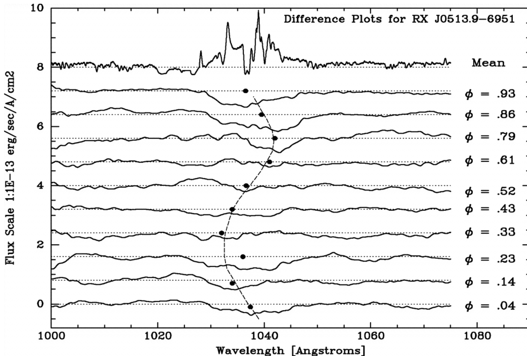
Fig. 5. from Far Ultraviolet Spectroscopic Explorer Observations of RX J0513.96951 Hutchings et al. 2005 AJ 129 2792 doi:10.1086/430147 https://dx.doi.org/10.1086/430147 © 2005. The American Astronomical Society. All rights reserved. Printed in U.S.A.
