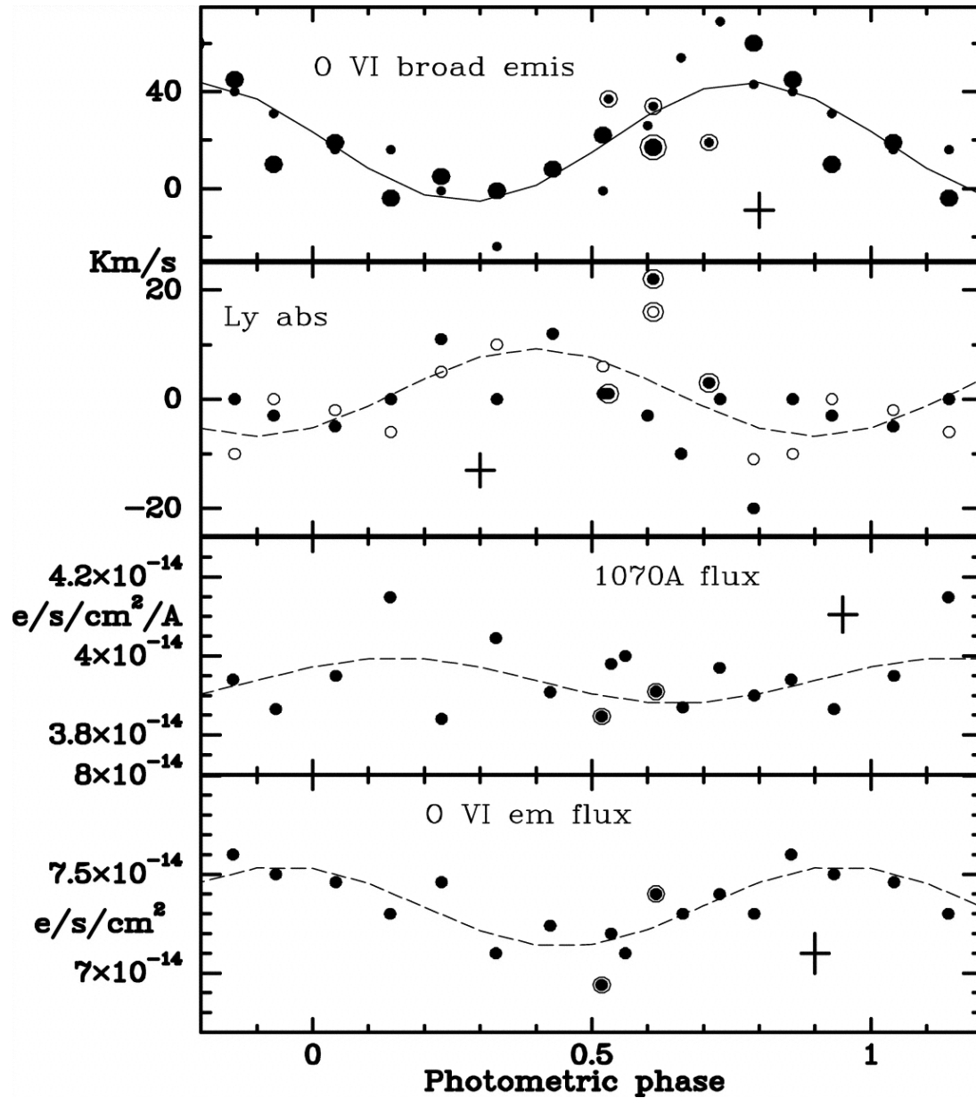
Fig. 4. from Far Ultraviolet Spectroscopic Explorer Observations of RX J0513.96951 Hutchings et al. 2005 AJ 129 2792 doi:10.1086/430147 https://dx.doi.org/10.1086/430147 © 2005. The American Astronomical Society. All rights reserved. Printed in U.S.A.
