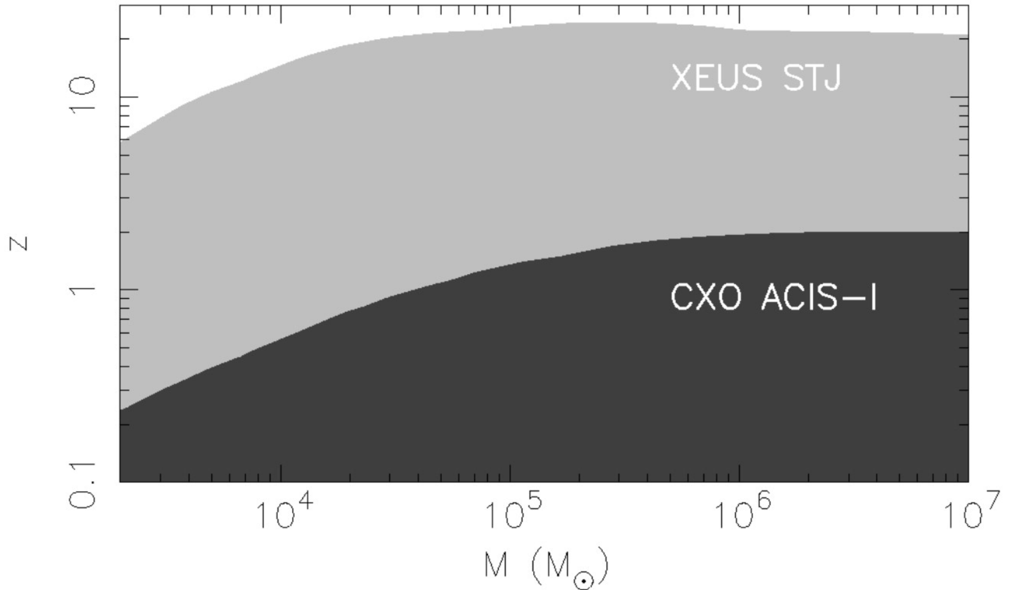
Fig. 2. from The Afterglow of Massive Black Hole Coalescence Milosavljević & Phinney 2005 ApJL 622 L93 doi:10.1086/429618 https://dx.doi.org/10.1086/429618
