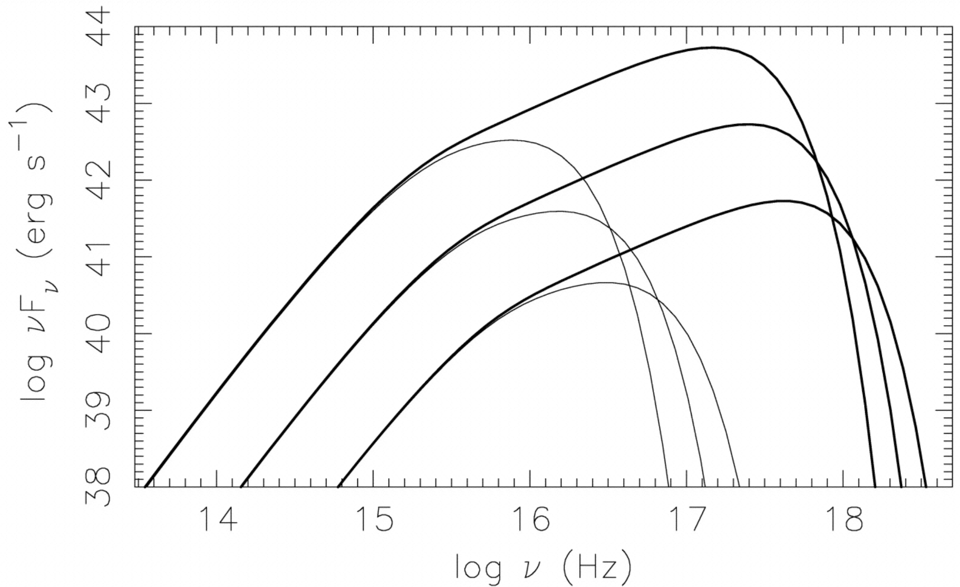
Fig. 1. from The Afterglow of Massive Black Hole Coalescence Milosavljević & Phinney 2005 ApJL 622 L93 doi:10.1086/429618 https://dx.doi.org/10.1086/429618
