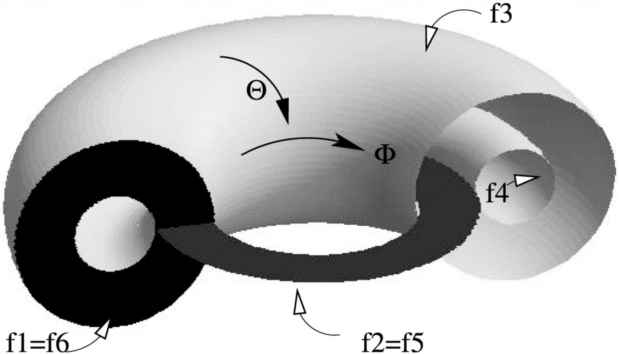
Fig. 3. from Magnetic Flux Tube Reconnection: Tunneling Versus Slingshot Linton & Antiochos 2005 ApJ 625 506 doi:10.1086/429585 https://dx.doi.org/10.1086/429585 © 2005. The American Astronomical Society. All rights reserved. Printed in U.S.A.
