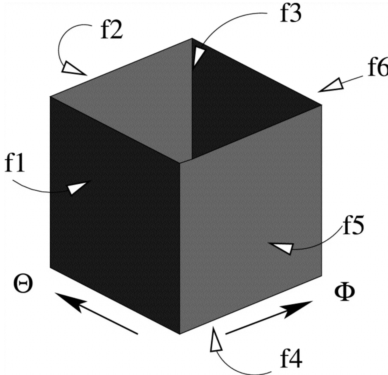
Fig. 3. from Magnetic Flux Tube Reconnection: Tunneling Versus Slingshot Linton & Antiochos 2005 ApJ 625 506 doi:10.1086/429585 https://dx.doi.org/10.1086/429585 © 2005. The American Astronomical Society. All rights reserved. Printed in U.S.A.
