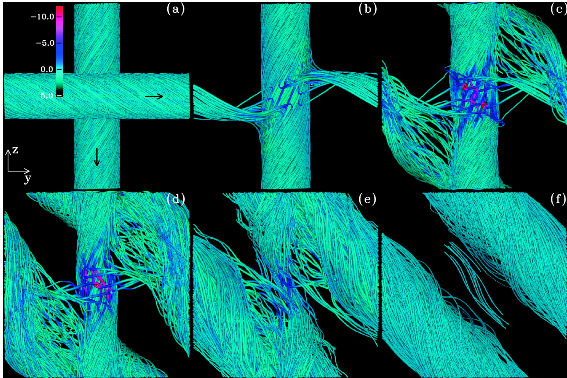
Fig. 1. from Magnetic Flux Tube Reconnection: Tunneling Versus Slingshot Linton & Antiochos 2005 ApJ 625 506 doi:10.1086/429585 https://dx.doi.org/10.1086/429585 © 2005. The American Astronomical Society. All rights reserved. Printed in U.S.A.
