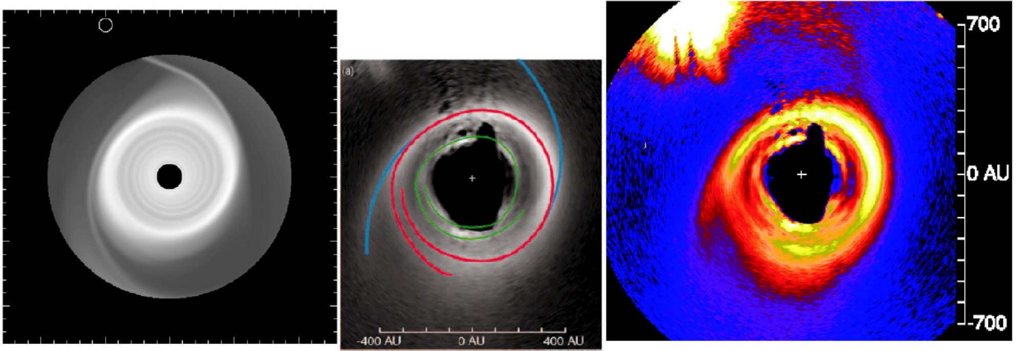
Fig. 7. from Driving Spiral Arms in the Circumstellar Disks of HD 100546 and HD 141569A Quillen et al. 2005 AJ 129 2481 doi:10.1086/428954 https://dx.doi.org/10.1086/428954 © 2005. The American Astronomical Society. All rights reserved. Printed in U.S.A.
