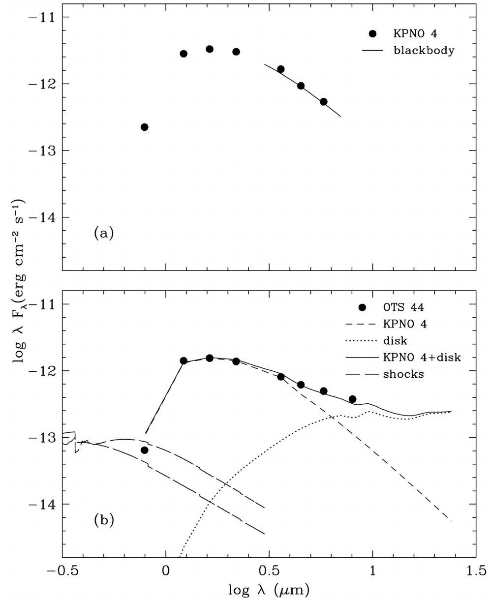
Fig. 1. from Spitzer Identification of the Least Massive Known Brown Dwarf with a Circumstellar Disk Luhman et al. 2005 ApJL 620 L51 doi:10.1086/428613 https://dx.doi.org/10.1086/428613
