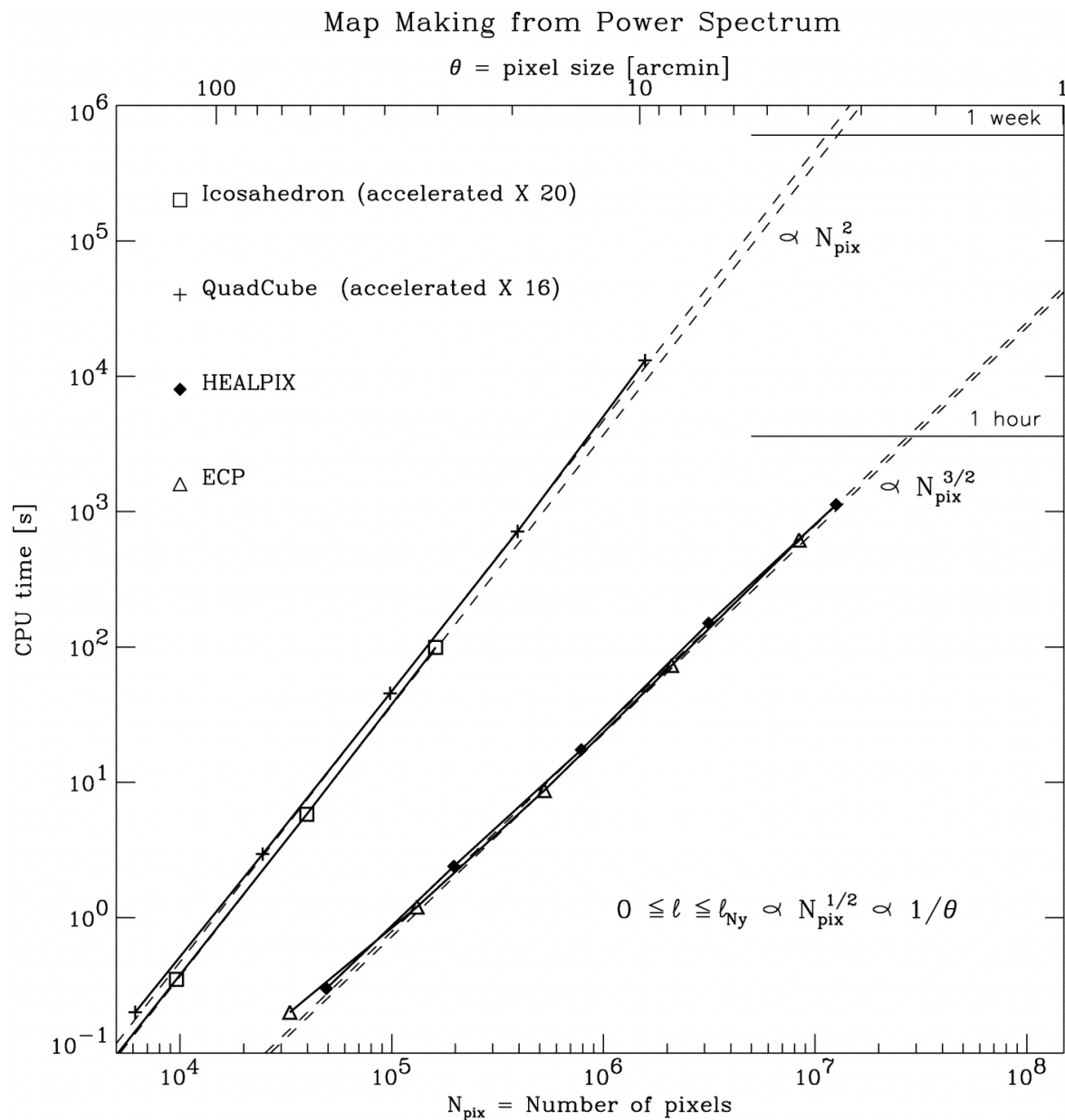
Fig. 7. from HEALPix: A Framework for HighResolution Discretization and Fast Analysis of Data Distributed on the Sphere Górski et al. 2005 ApJ 622 759 doi:10.1086/427976 https://dx.doi.org/10.1086/427976
