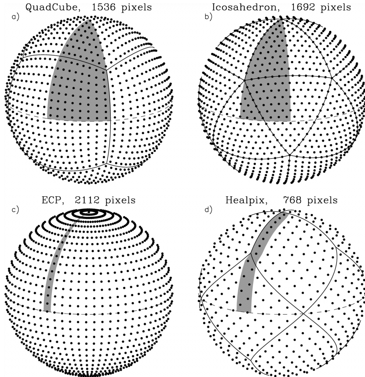
Fig. 6. from HEALPix: A Framework for HighResolution Discretization and Fast Analysis of Data Distributed on the Sphere Górski et al. 2005 ApJ 622 759 doi:10.1086/427976 https://dx.doi.org/10.1086/427976
