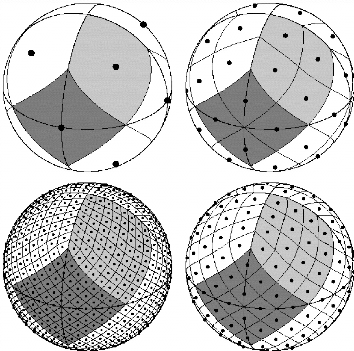
Fig. 3. from HEALPix: A Framework for HighResolution Discretization and Fast Analysis of Data Distributed on the Sphere Górski et al. 2005 ApJ 622 759 doi:10.1086/427976 https://dx.doi.org/10.1086/427976 © 2005. The American Astronomical Society. All rights reserved. Printed in U.S.A.
