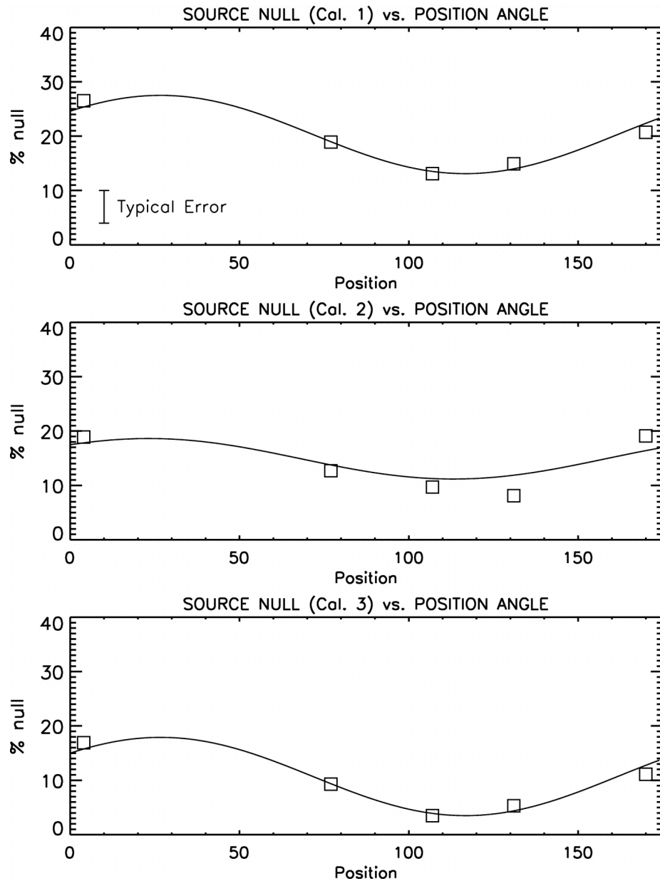
Fig. 1. from Resolved MidInfrared Emission around AB Aurigae and V892 Tauri with Adaptive Optics Nulling Interferometric Observations Liu et al. 2005 ApJL 618 L133 doi:10.1086/427922 https://dx.doi.org/10.1086/427922
