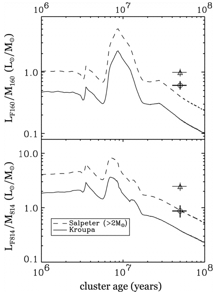
Fig. 5. from Mass Segregation and the Initial Mass Function of Super Star Cluster M82F McCrady, Graham, & Vacca 2005 ApJ 621 278 doi:10.1086/427487 https://dx.doi.org/10.1086/427487
