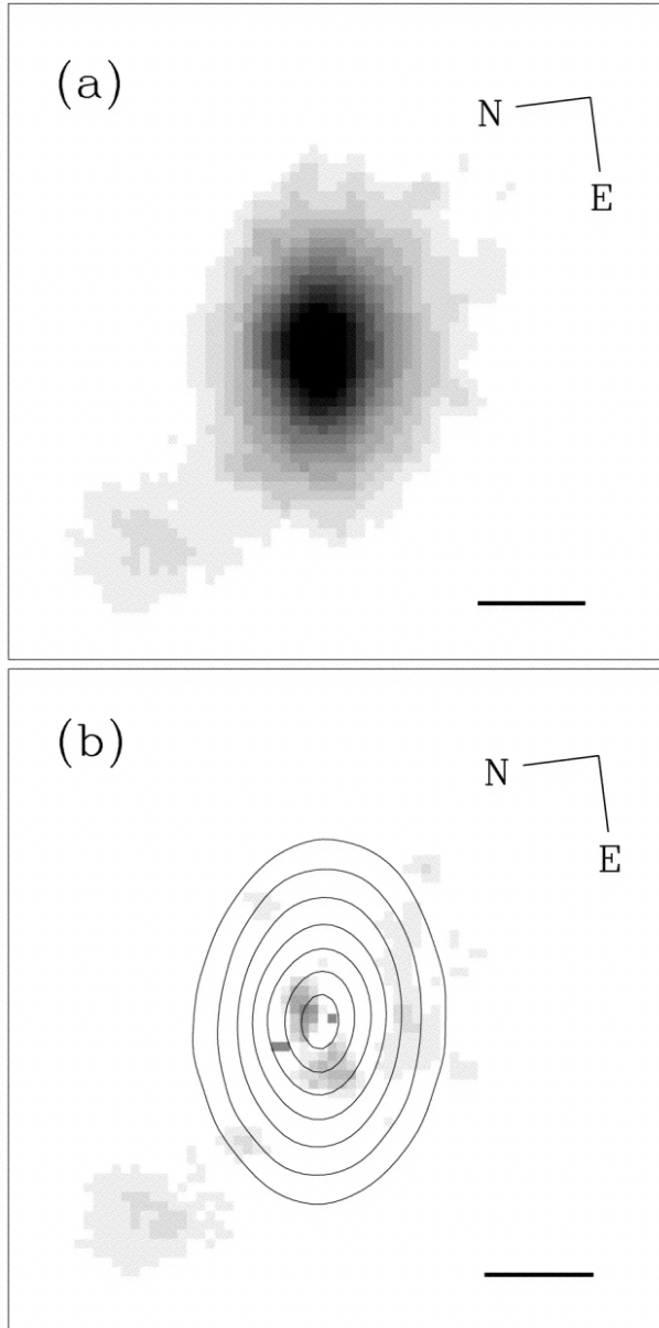
Fig. 3. from Mass Segregation and the Initial Mass Function of Super Star Cluster M82F McCrady, Graham, & Vacca 2005 ApJ 621 278 doi:10.1086/427487 https://dx.doi.org/10.1086/427487 © 2005. The American Astronomical Society. All rights reserved. Printed in U.S.A.
