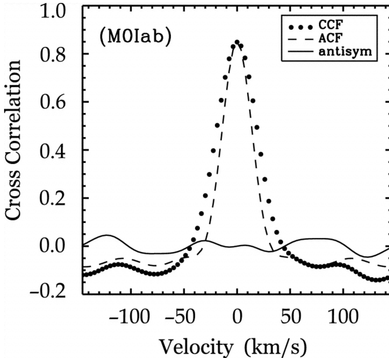
Fig. 2. from Mass Segregation and the Initial Mass Function of Super Star Cluster M82F McCrady, Graham, & Vacca 2005 ApJ 621 278 doi:10.1086/427487 https://dx.doi.org/10.1086/427487
