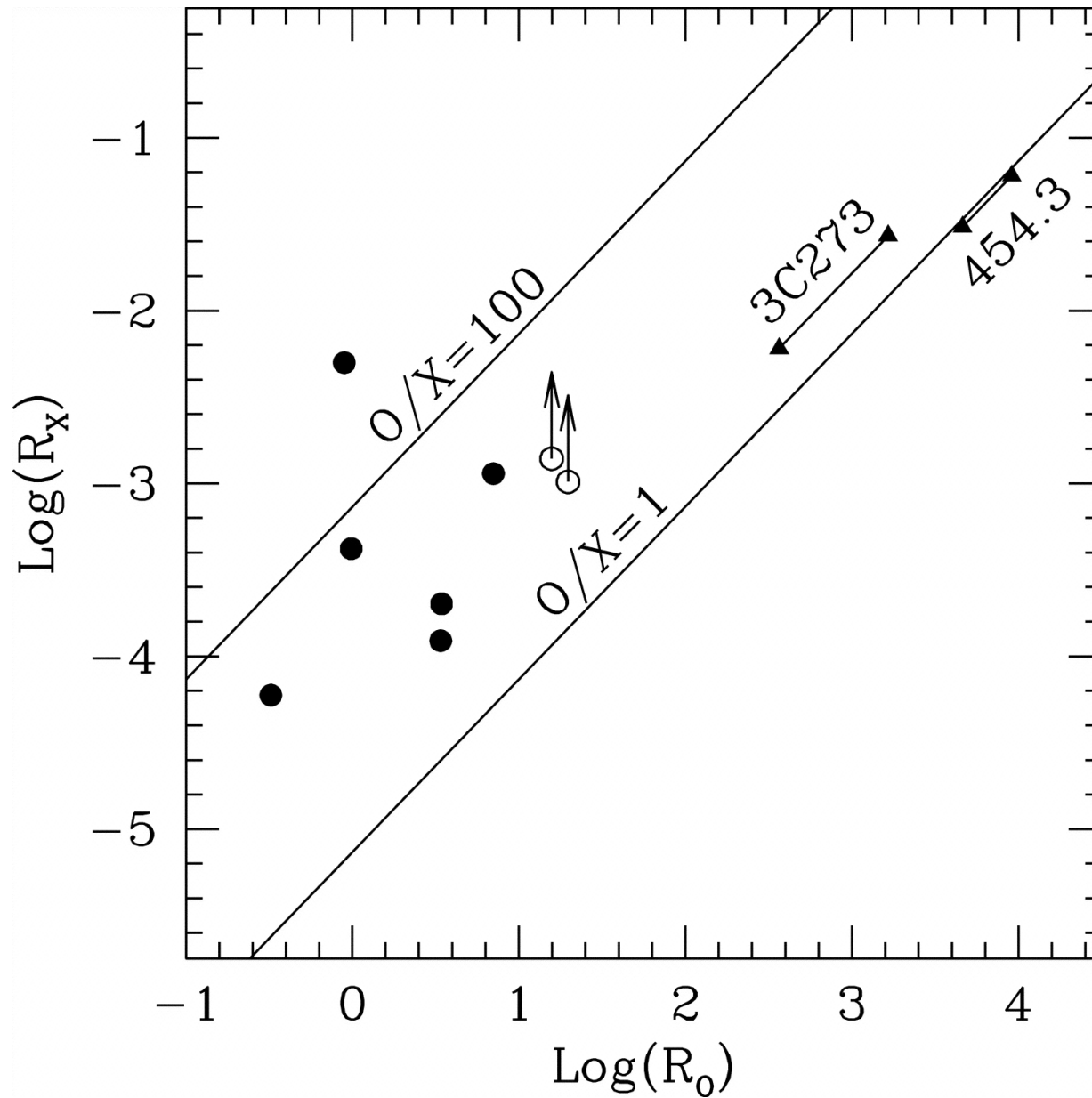
Fig. 3. from VLBA Imaging of Central Engines in RadioQuiet Quasars Ulvestad, Antonucci, & Barvainis 2005 ApJ 621 123 doi:10.1086/427426 https://dx.doi.org/10.1086/427426
